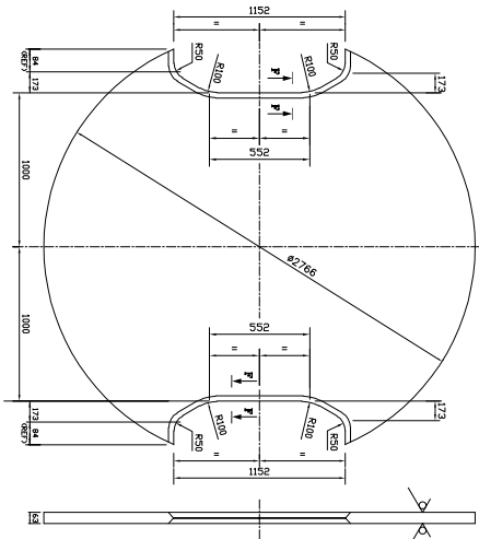
PLAN DETAIL OF ITEM 01
