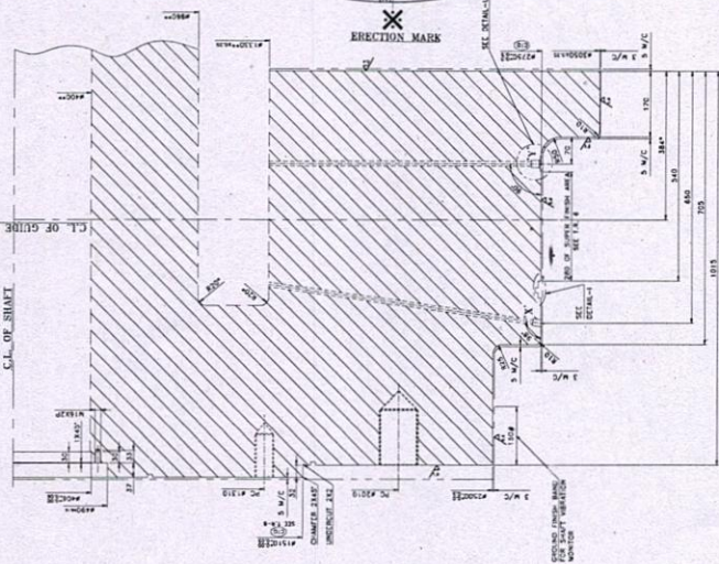
ENLARGED DETAIL-M
