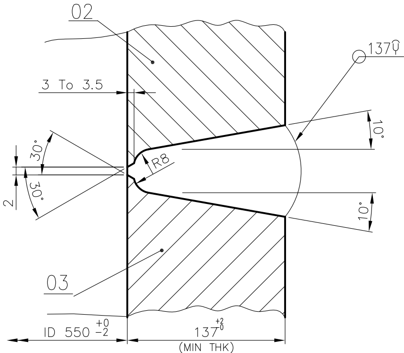
DETAIL-C
