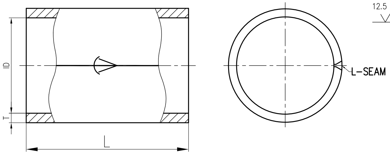
CHANNEL SHELL
