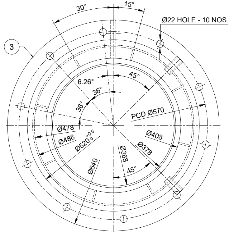
VIEW - A
