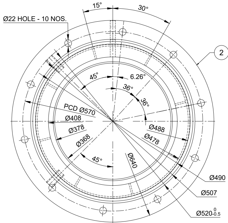
VIEW - B
