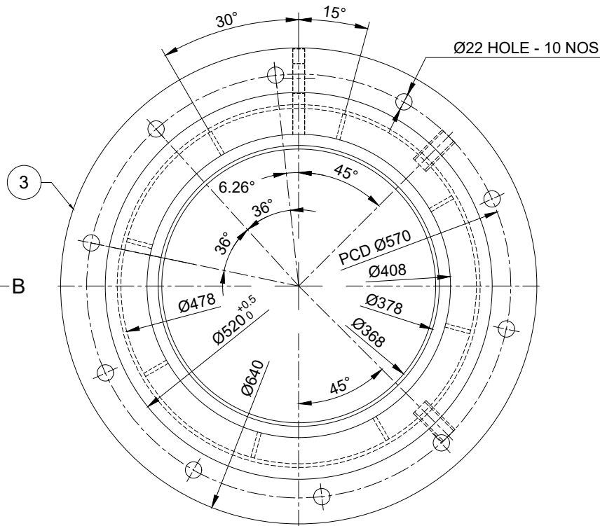
VIEW - A
