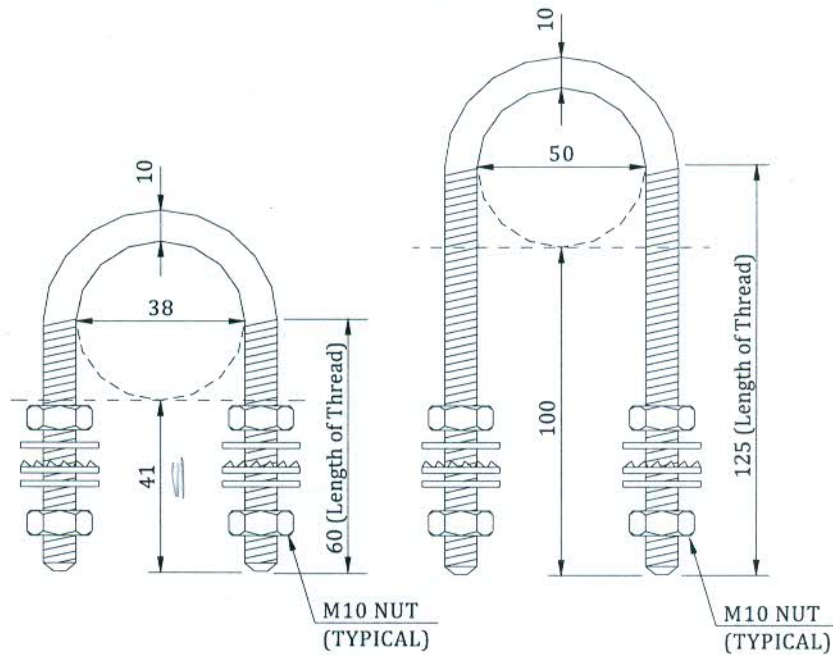
U-BOLT - 1 Material SS-304
