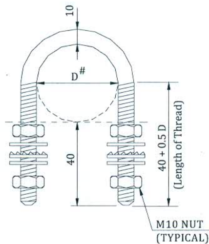
U-BOLT - 3 Material SS-304
