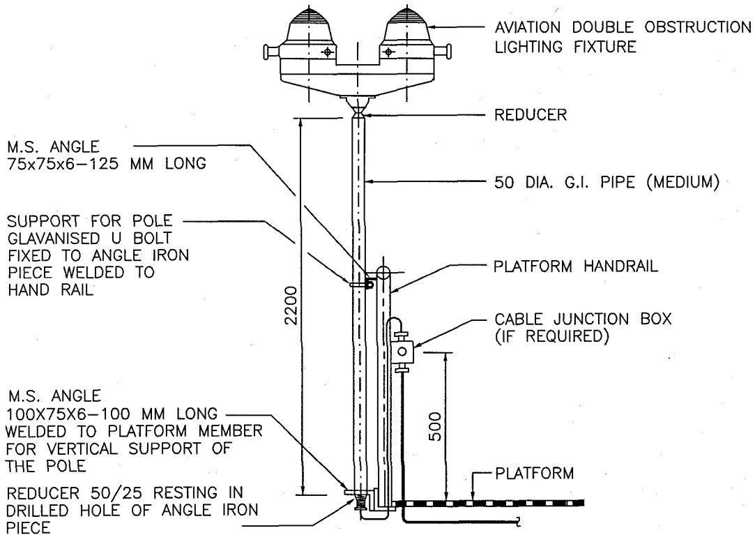
MOUNTED ON TOP OF STRUCTURE PLATFORM DETAIL-1
