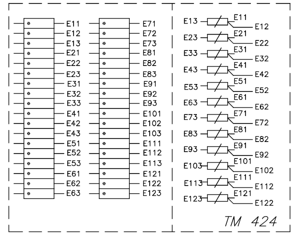
CONNECTION DIAGRAM FOR 12 NOS. WINDING ETDS. (SIMPLEX TYPE)
