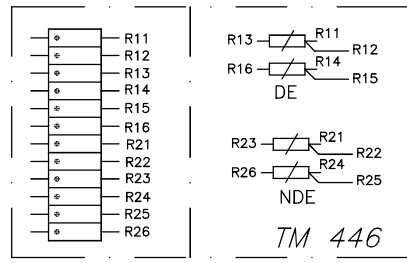
CONNECTION DIAGRAM FOR BRG. RTDS. (DUPLIX TYPE)
