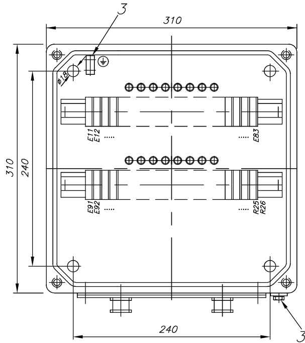
VIEW FROM - Z WITH COVER REMOVED
