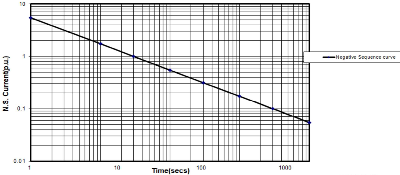
Curve No. 43113-61-05
