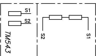
CONNECTION DIAGRAM FOR SPACE HEATERS
