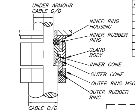
DOUBLE COMPRESSION TYPE CABLE GLAND (BRASS NICKEL PLATED)
