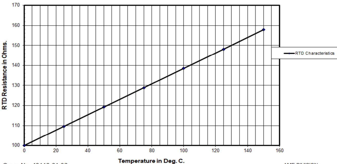
Curve No. 43113-61-06
