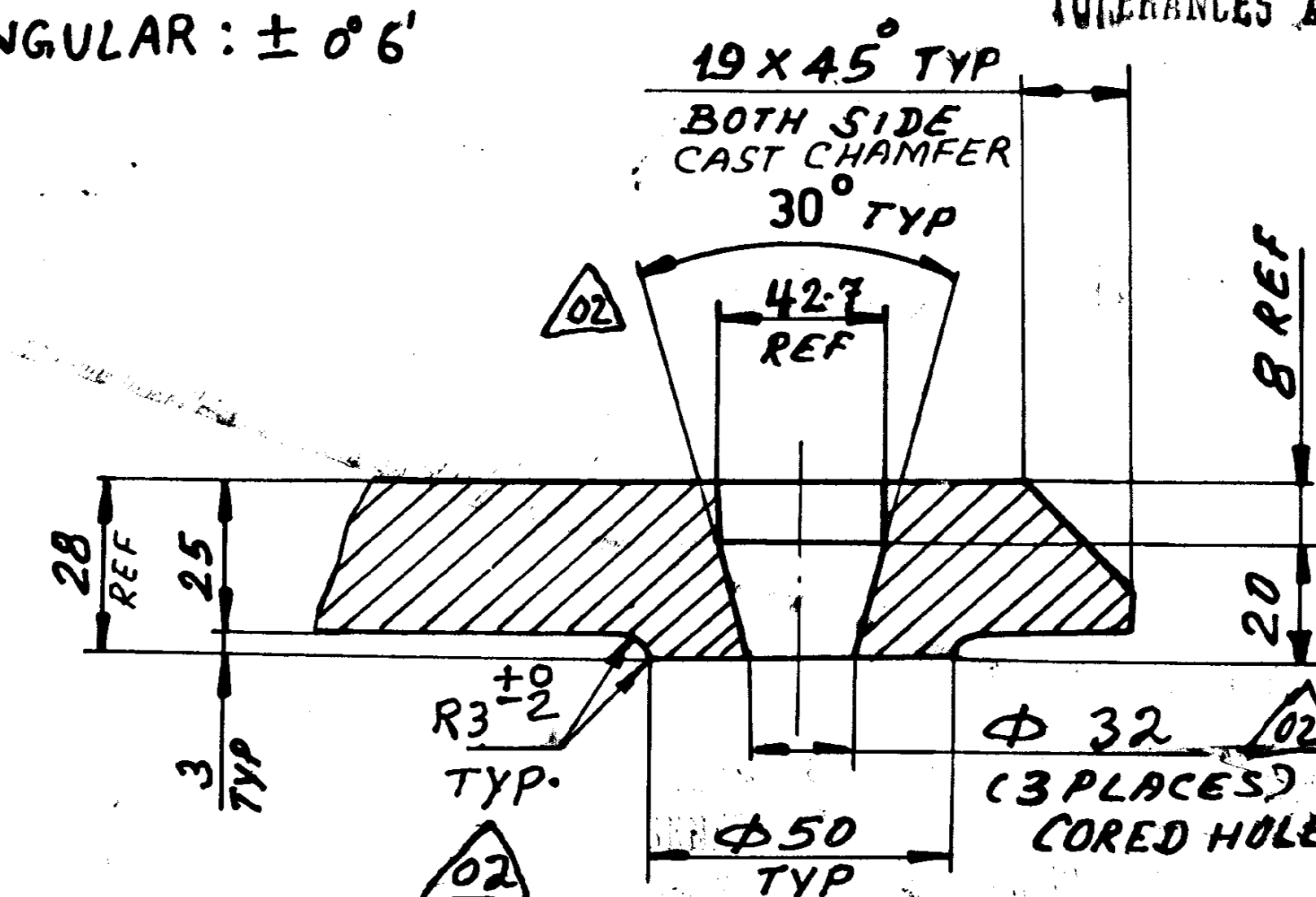
SECTION - AA
