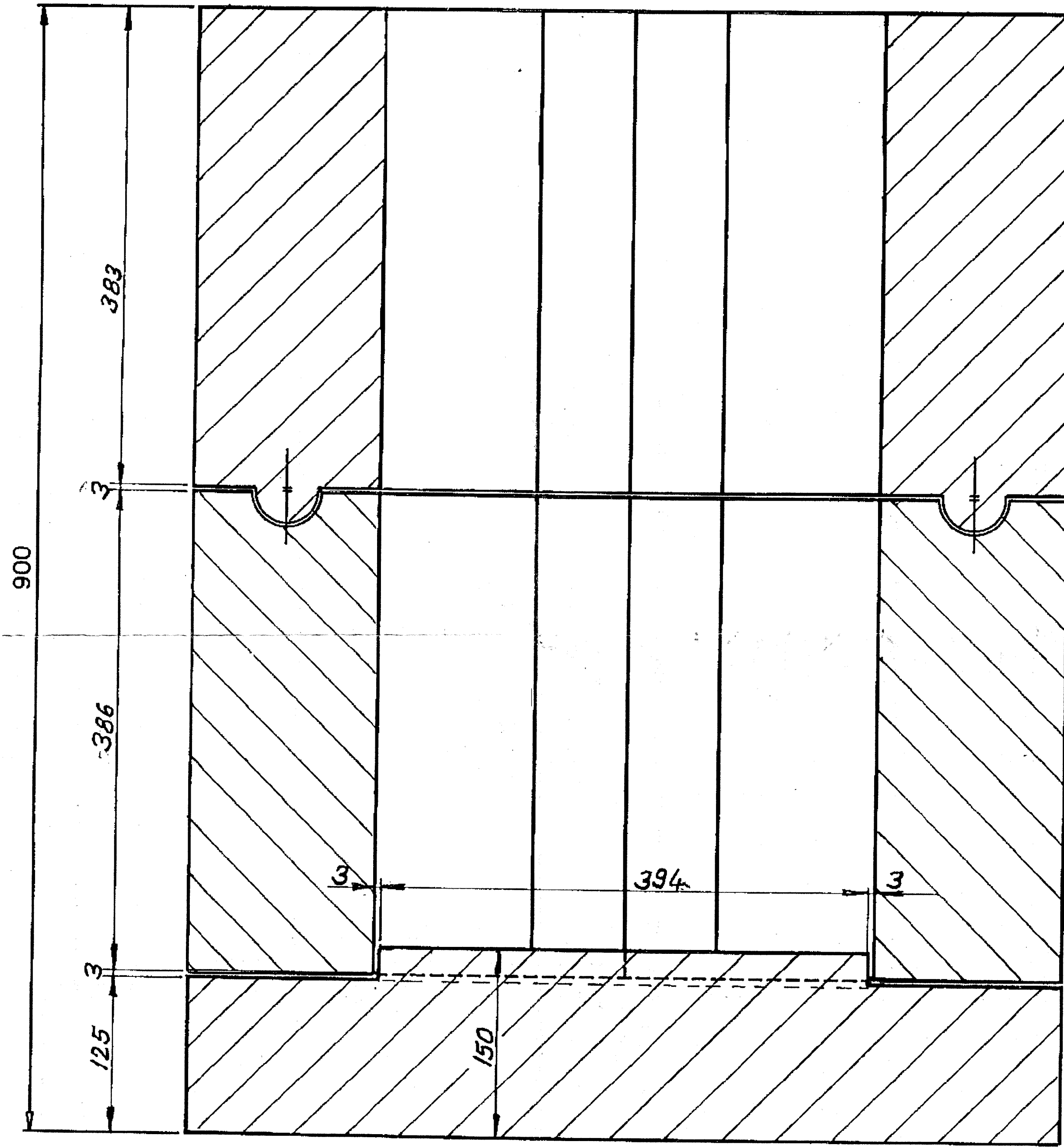
SECTION-BB
