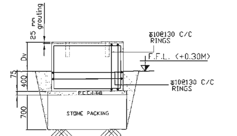
SECTION E-E
