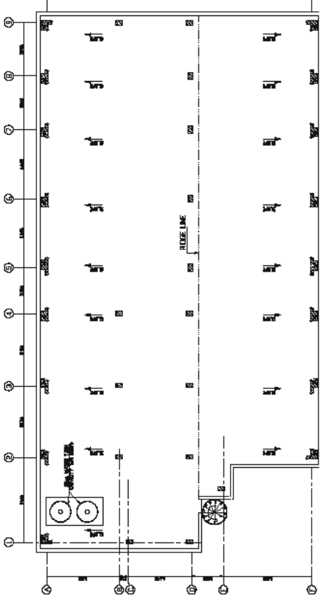
TERRACE PLAN
