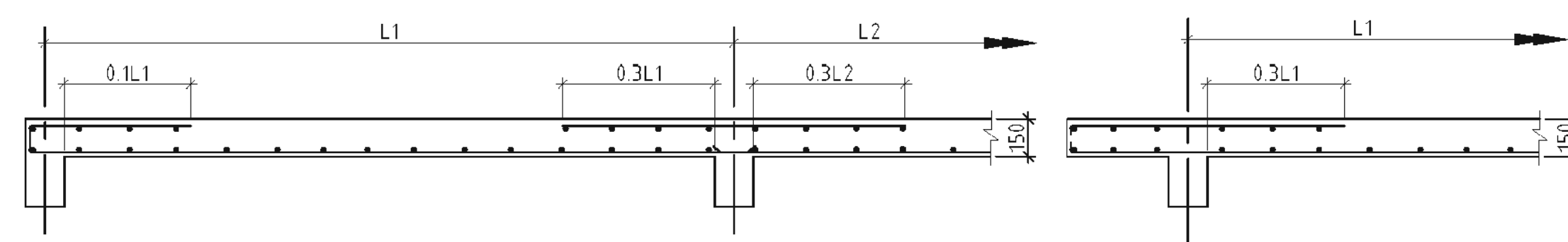
TYPICAL CURTAILMENT DETAIL OF SLAB BARS
