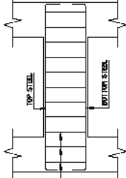
TYP. LONGITUDINAL SECTION FOR LINTELS (ONE SIDE BRICK WALL SUPPORT & OTHER SIDE COLUMN SUPPORT)
