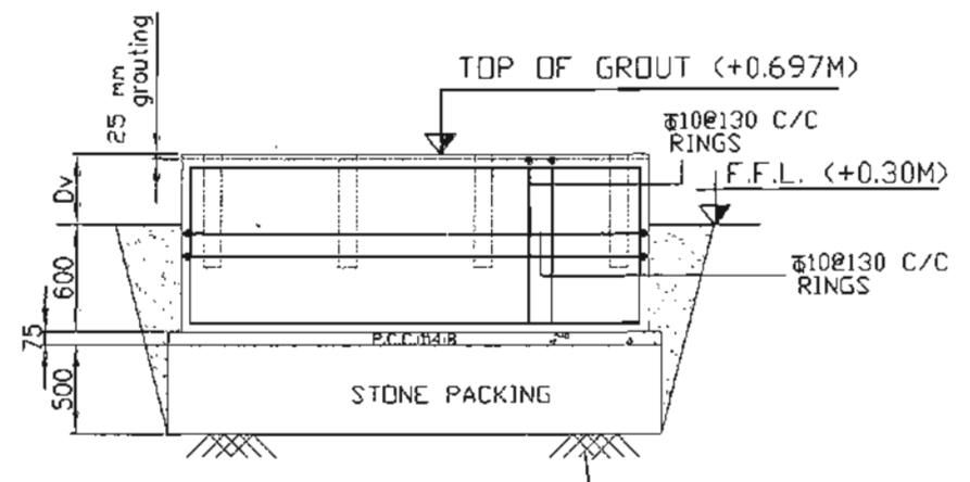
SECTION C-C
