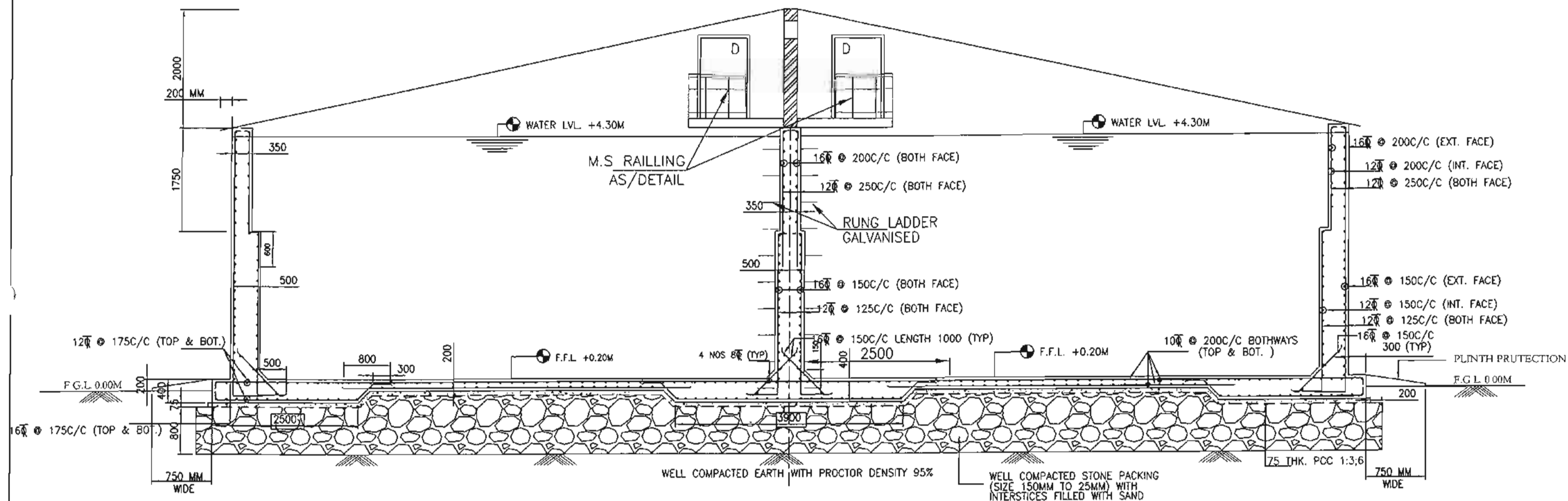
SECTION 1-1
