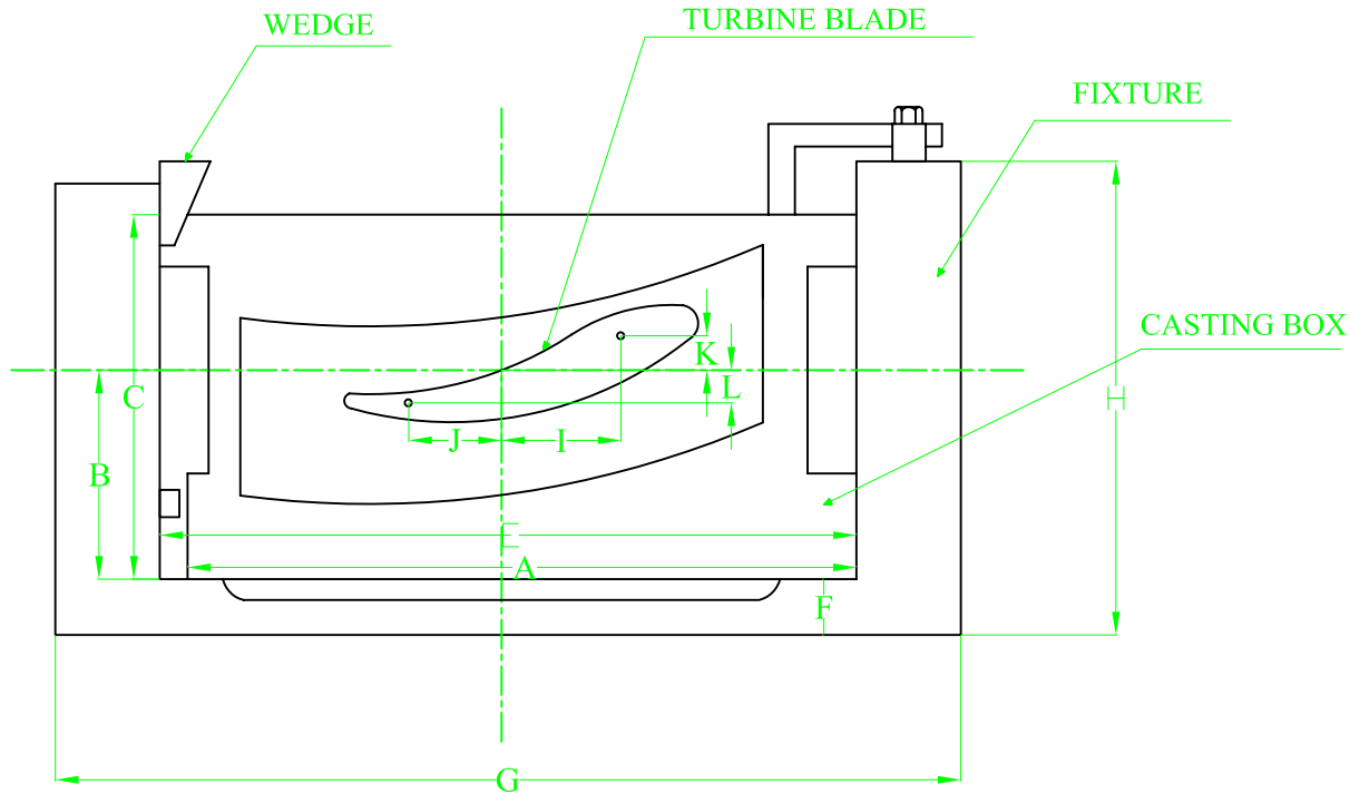
VIEW OF LEFT HAND BLADE
