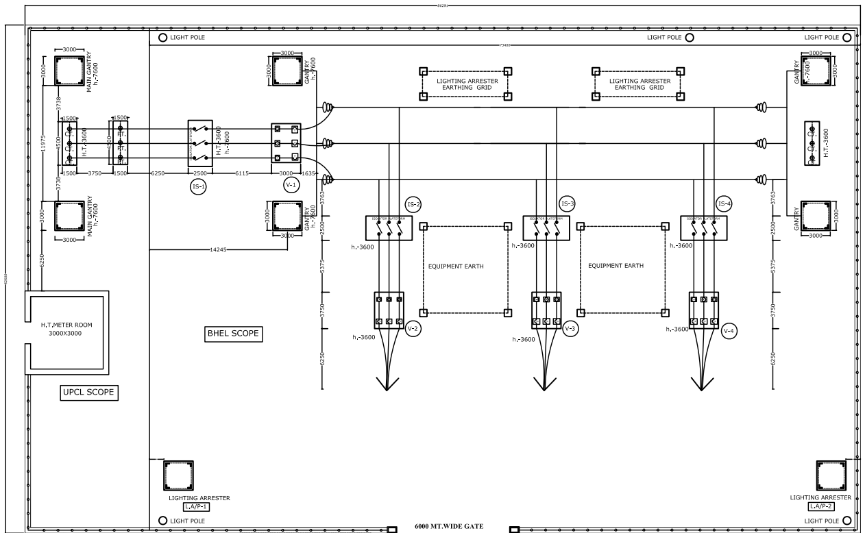
PLAN OF 33/0.4 KV -(4MVA X2NOS.)8MVA SUB STATION
