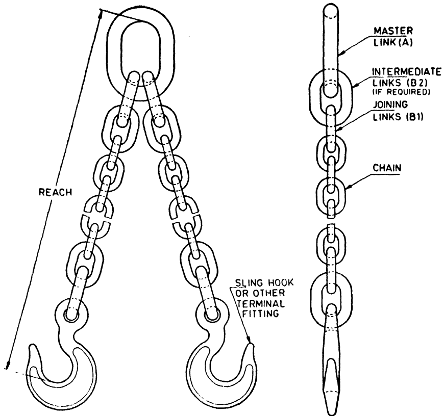
FIG. 2 TWO-LEO SLING
