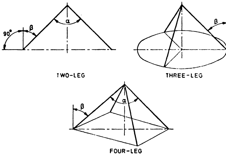
FIG. 5 INCLINATION OF SLING LEGS
