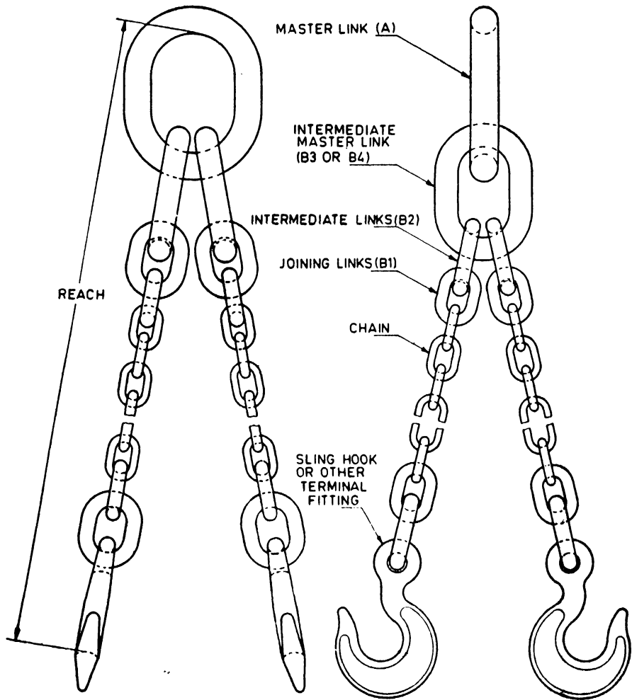
FIG. 4 FOUR-LEO SLING
