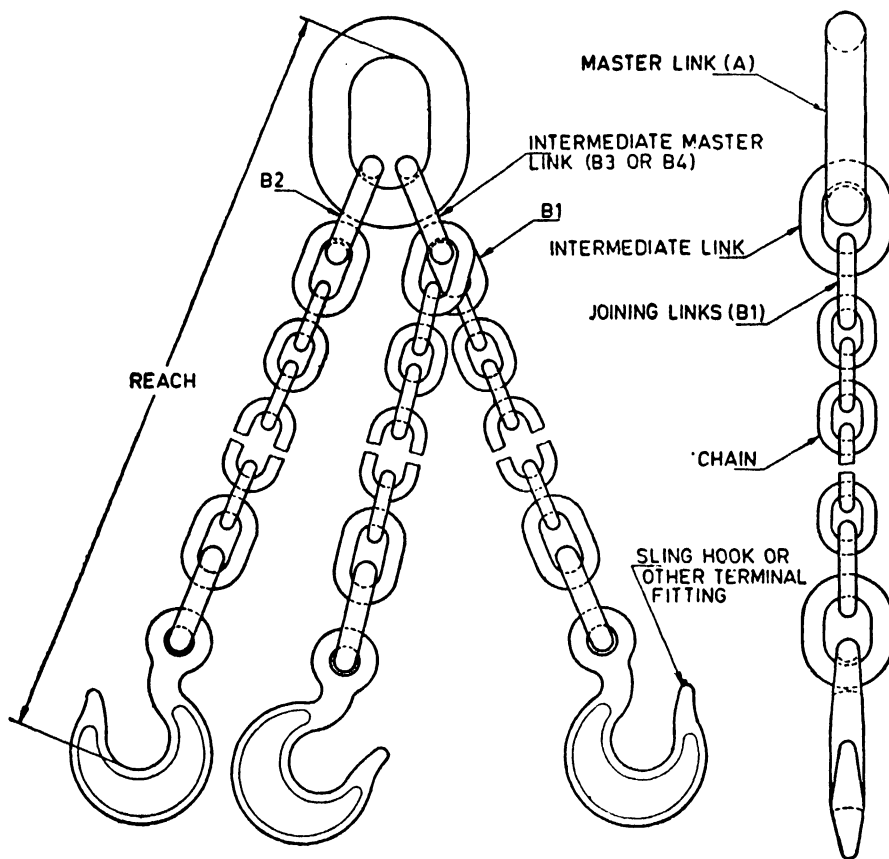
FIG. 3 THREE-LEO SLING
