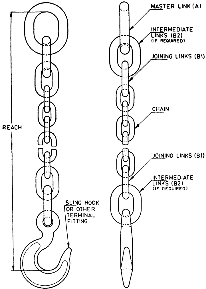
FIG. 1 SINGLE-LEO SLING
