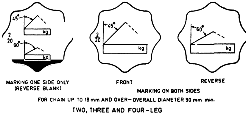
FIG. 6 EXAMPLES OF MARKING TAGS
