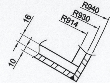
ENLARGE VIEW - X
