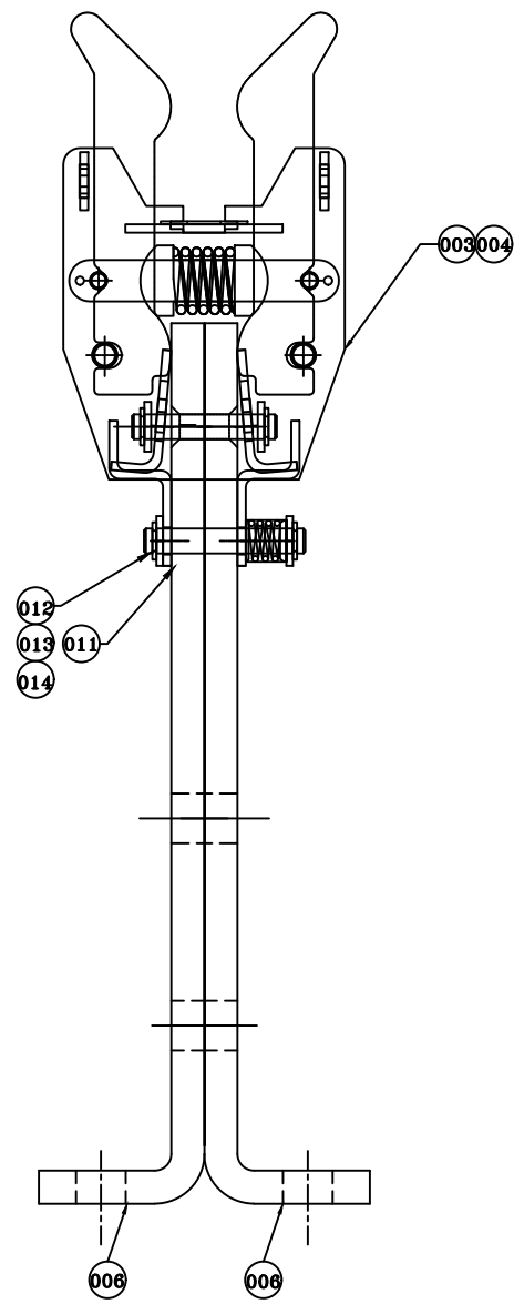
VAR. 02 & 03 (2NOS.-8TK. x 100 WIDE CONNECTOR)
