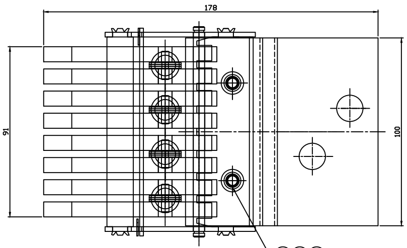
VAR. 02 & 03 (2NOS.-8TK. x 100 WIDE CONNECTOR)
