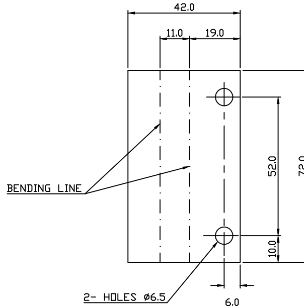
DEVELOPMENT OF ITEM 001
