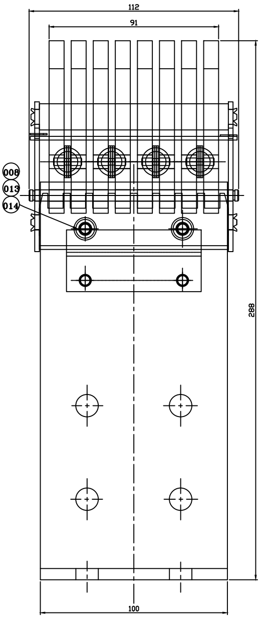
VAR. 02 & 03 (2NOS.-8TK. x 100 WIDE CONNECTOR)
