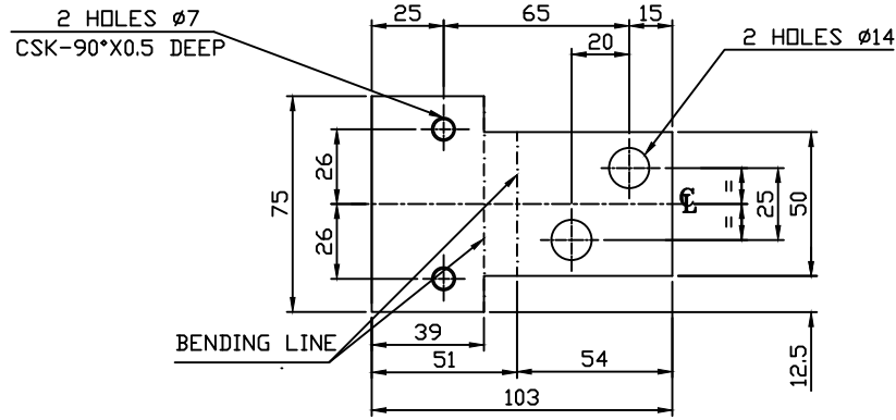
DEVELOPMENT OF IT. 002
