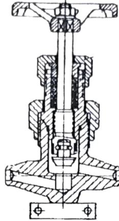
Schematic Diagram of Control/Stop Valve
