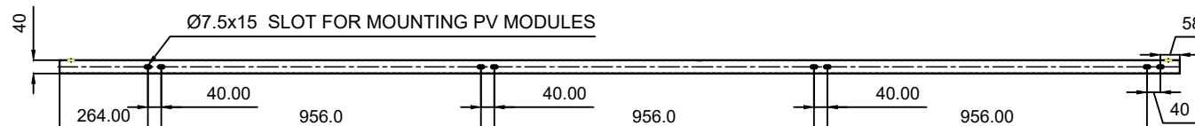
TOP VIEW
