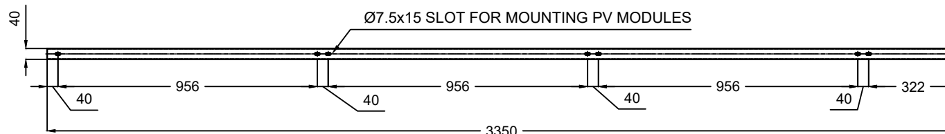
TOP VIEW
