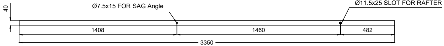
BOTTOM VIEW
