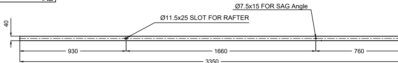
BOTTOM VIEW
