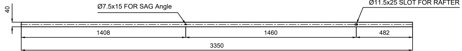
BOTTOM VIEW
