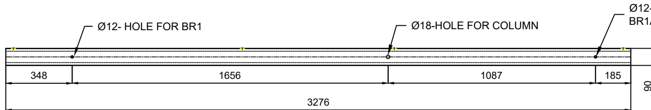
FRONT VIEW
