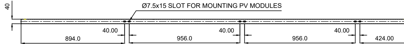
FRONT VIEW
