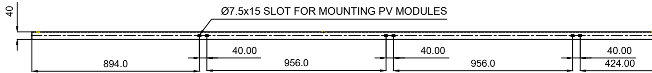
FRONT VIEW
