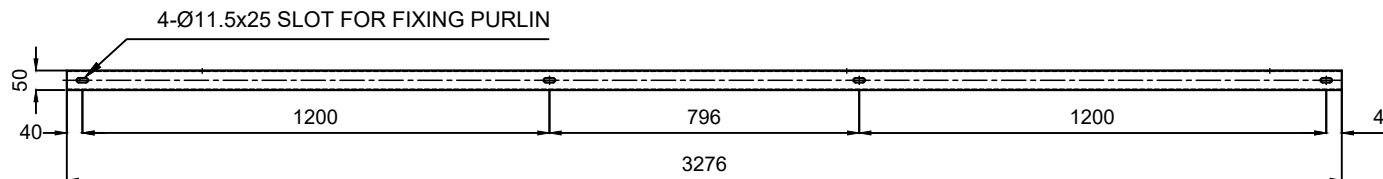
TOP VIEW
