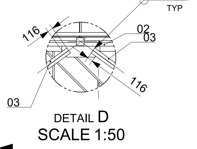
DETAIL D SCALE 1:50
