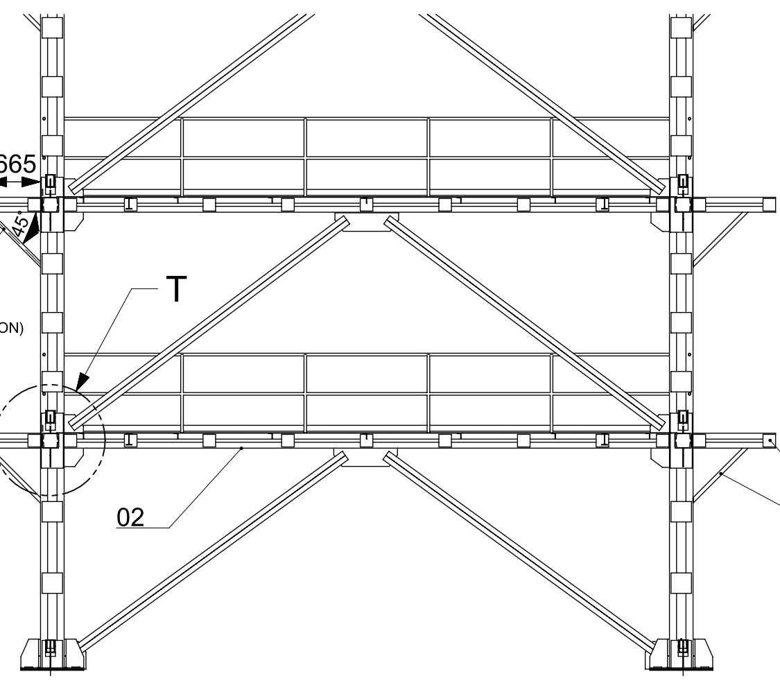
SECTION S-S
