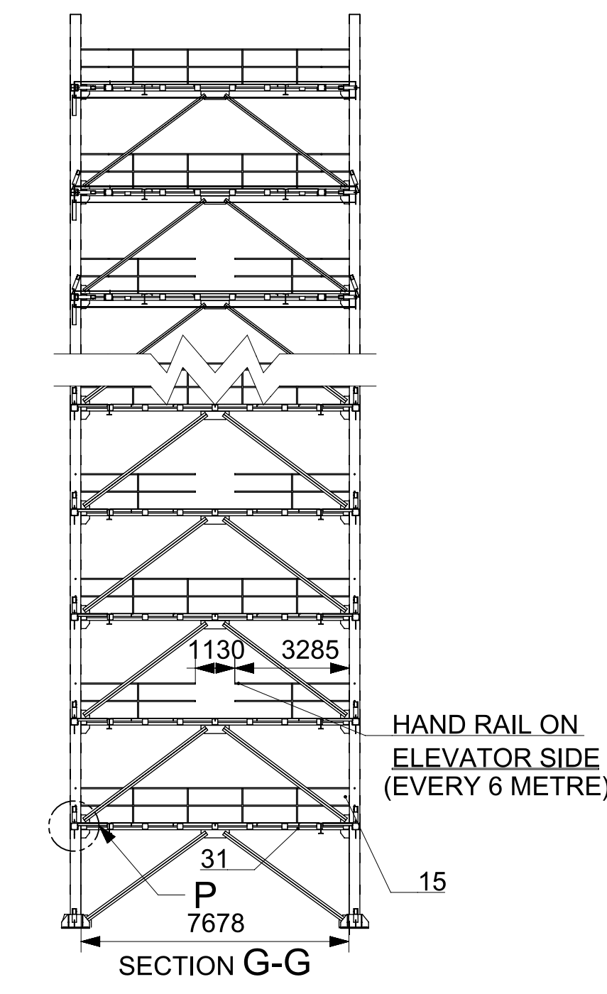
SECTION G-G
