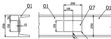
TYPICAL JOINT DETAIL
