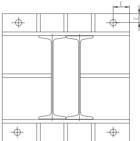
BASE PLATE DETAIL FOR UB/NPB BOX (FOR 4-BOLT)
