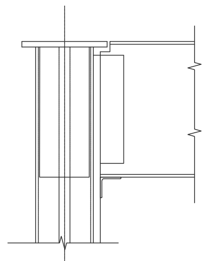
COLUMN-BEAM CONNECTION
