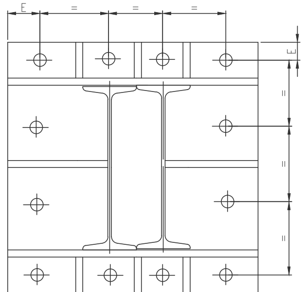
BASE PLATE DETAIL FOR UB/NPB BOX (FOR 12-BOLT)
