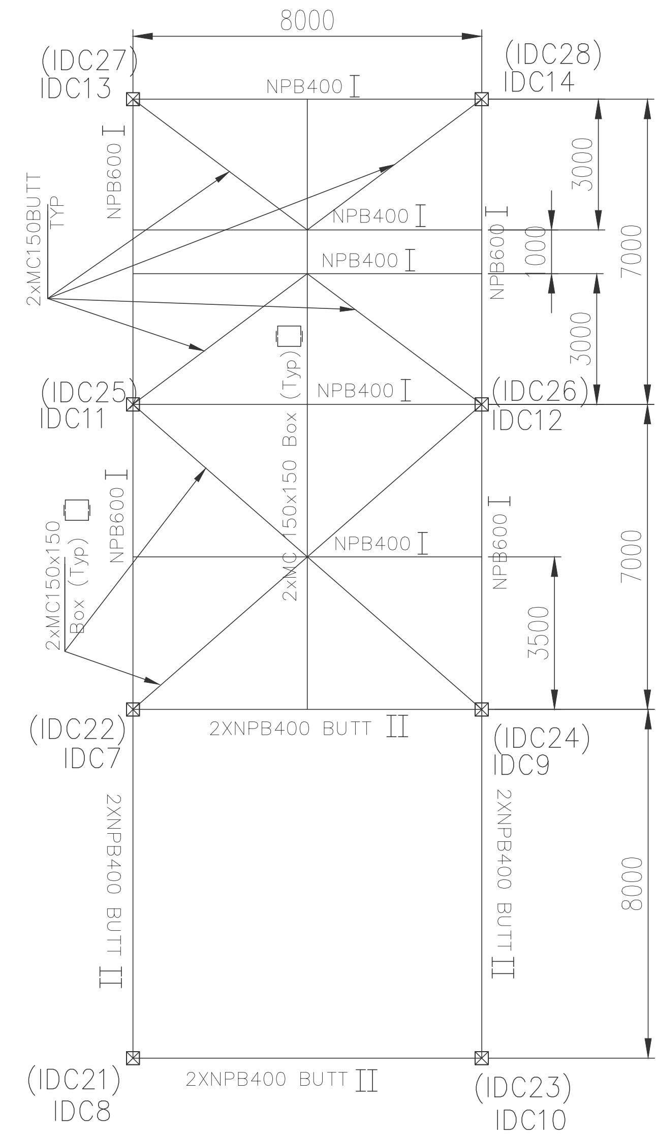
Plan @ EL+36.550M(TOS)
