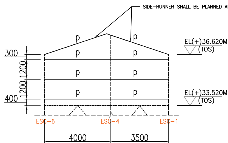
LOCATION OF SIDE–RUNNER ABOVE EL+33.520M (FOR MACHINE ROOM)
