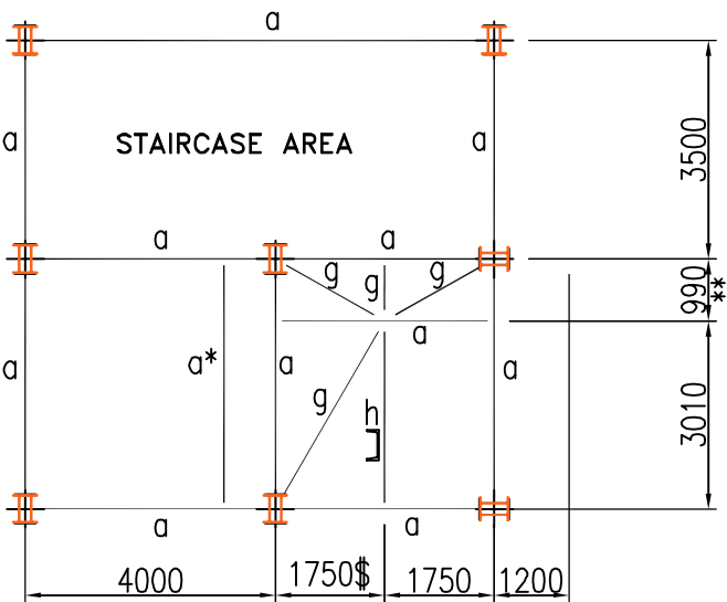
PLAN @ EL(+) 15.400M EL(+) 30.780M (STAIRCASE IS NOT SHOWN FOR CLARITY)
