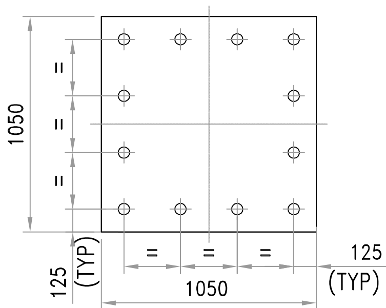
(FOR 12–BOLT) BASE PLATE DETAILS
