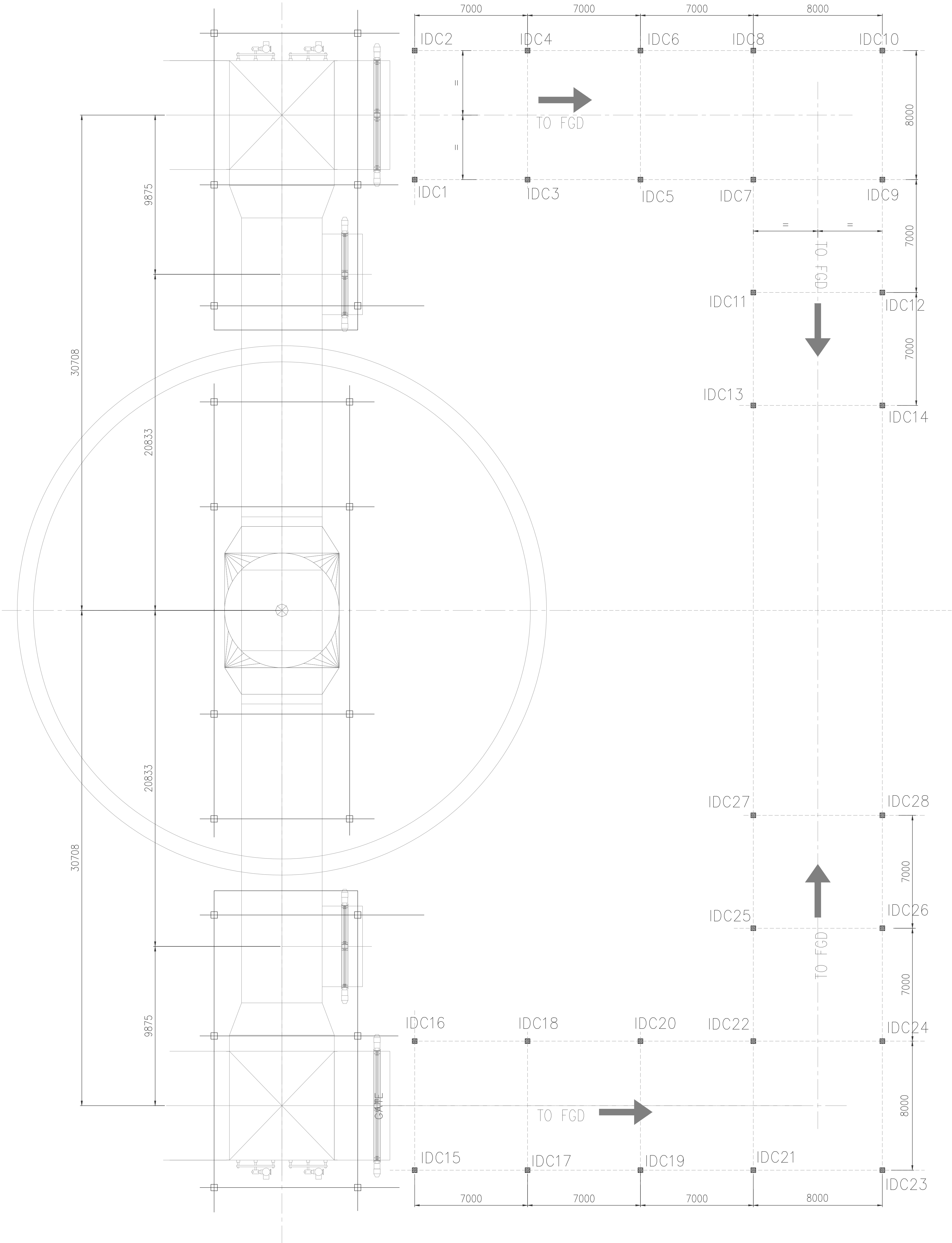
LOCATION OF FGD INLET DUCT COLUMNS
