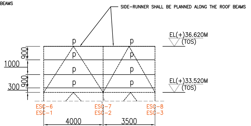
LOCATION OF SIDE–RUNNER ABOVE EL+33.120M (FOR MACHINE ROOM)
