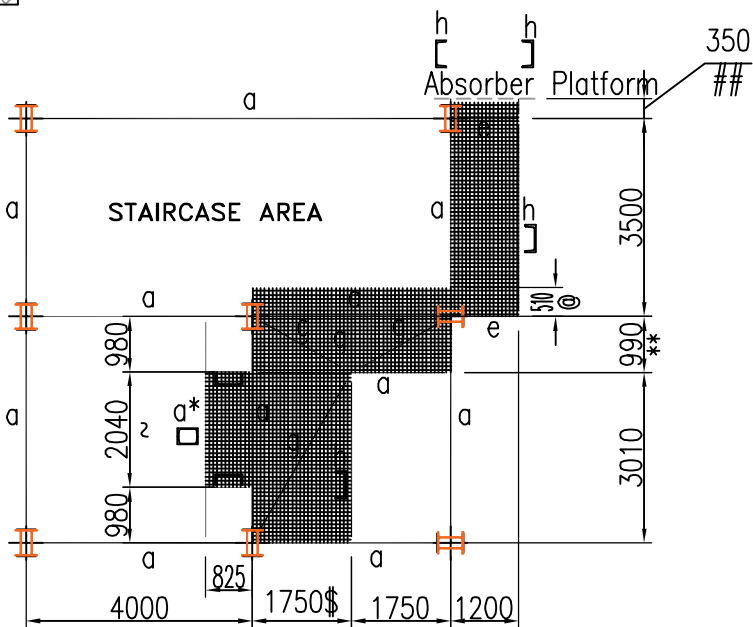
PLAN @ EL(+).11.300M (INCLUDING PLATFORMS) (STAIRCASE IS NOT SHOWN FOR CLARITY)
