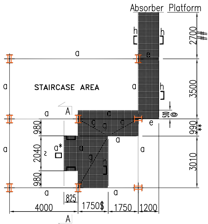
PLAN @ EL(+).3.700M EL(+).6.500M EL(+).18.800M EL(+).24.210M EL(+).28.220M (INCLUDING PLATFORMS) (STAIRCASE IS NOT SHOWN FOR CLARITY)
