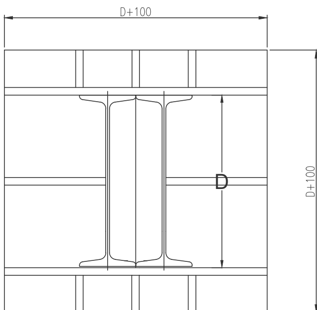
CAP PLATE DETAIL FOR UB/NPB BOX COLUMNS
