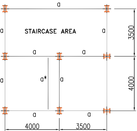
PLAN @ EL(+) 2.400M EL(+) 8.900M EL(+) 22.300M (STAIRCASE IS NOT SHOWN FOR CLARITY)
