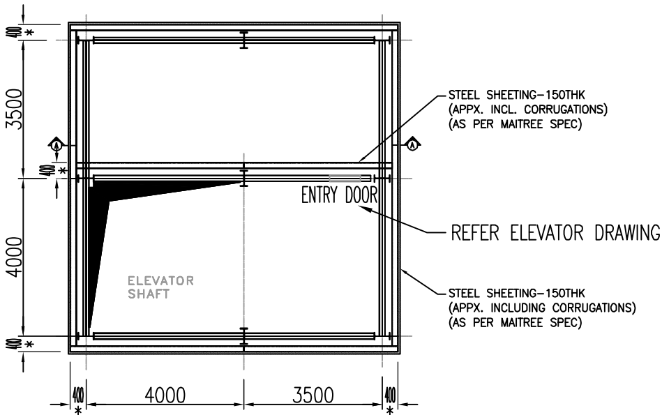
PURLIN WITH STEEL SHEETING PLAN VIEW (FOR ELEVATOR MACHIN ROOM) (NOTE: STAIRCASE SHOWN IS INDICATIVE ONLY)
