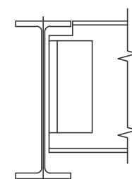
BEAM-BEAM CONNECTION
