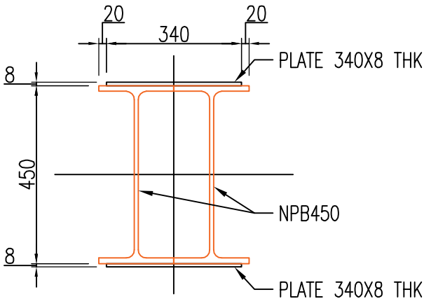
DETAIL OF COLUMN 'C1'
