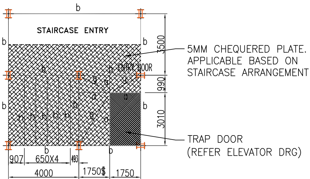
PLAN @ EL(+).33.120M (STAIRCASE IS NOT SHOWN FOR CLARITY)
