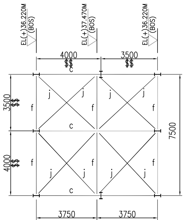
ROOF BEAM/BRACING PLAN VIEW @EL+36.220m(END) to EL+37.470M(MID)
