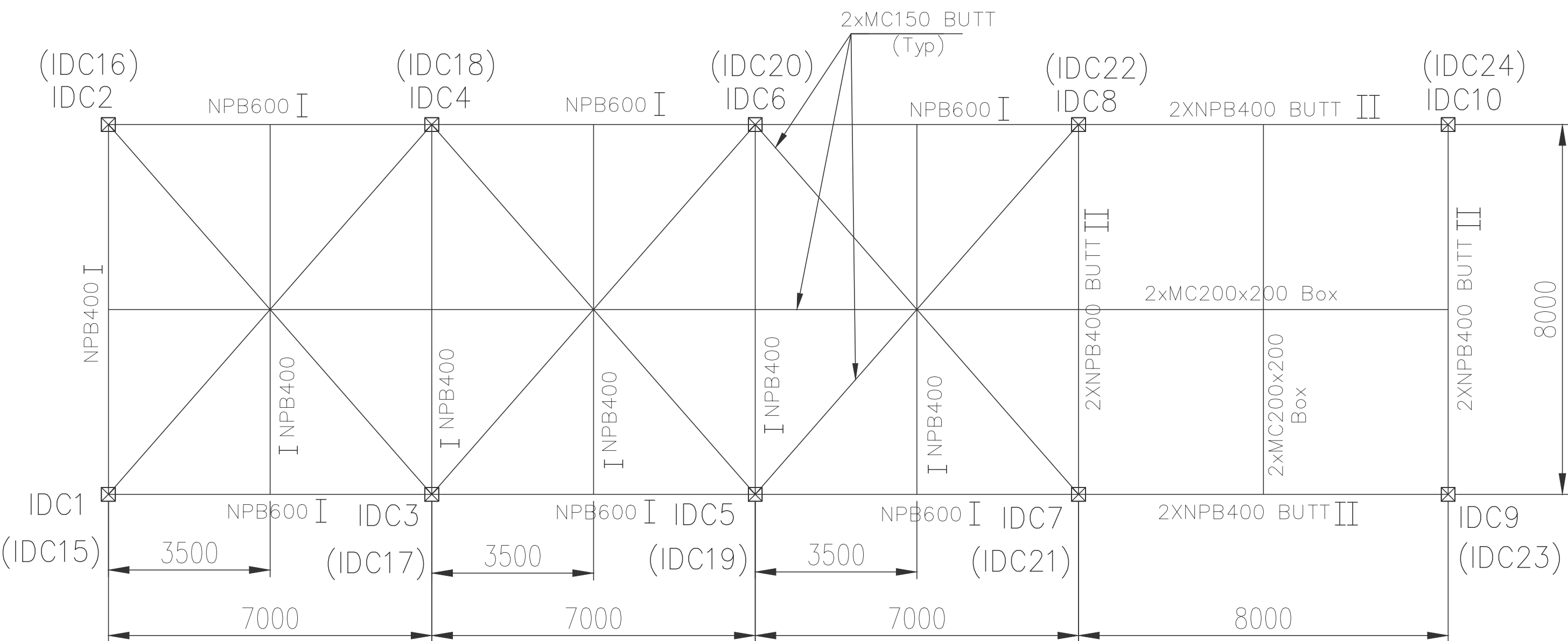
Plan @ EL+1.6M (TOS)
