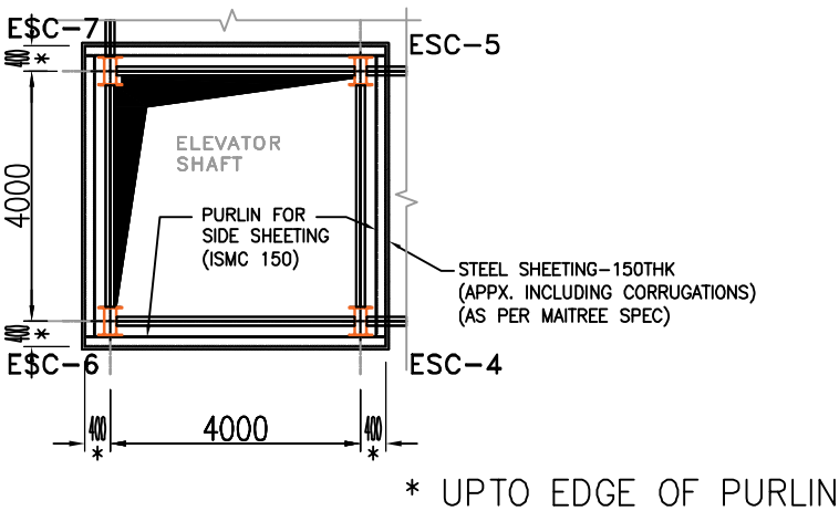
PURLIN WITH STEEL SHEETING PLAN VIEW (FOR ELEVATOR SHAFT)
