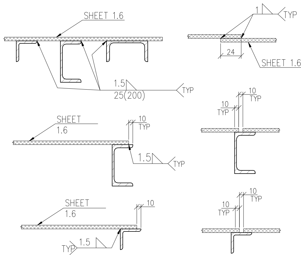
TYP. WELDING DETAILS OF SHEET 1.6MM
