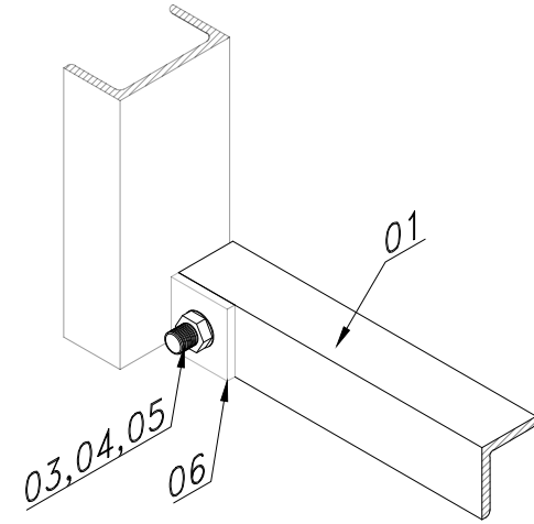
DETAIL - 'X' (MOUNTING PLATE ARRANGEMENT) (TYP.)
