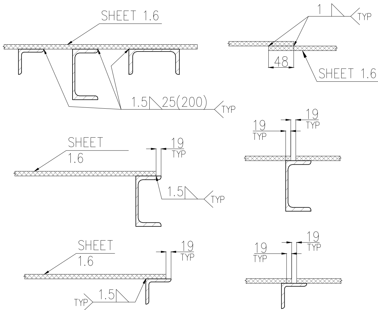
TYP. WELDING DETAILS OF SHEET 1.6MM
