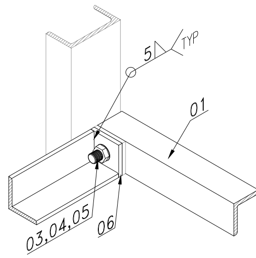
DETAIL - 'Y' (MOUNTING PLATE ARRANGEMENT) (TYP.)
