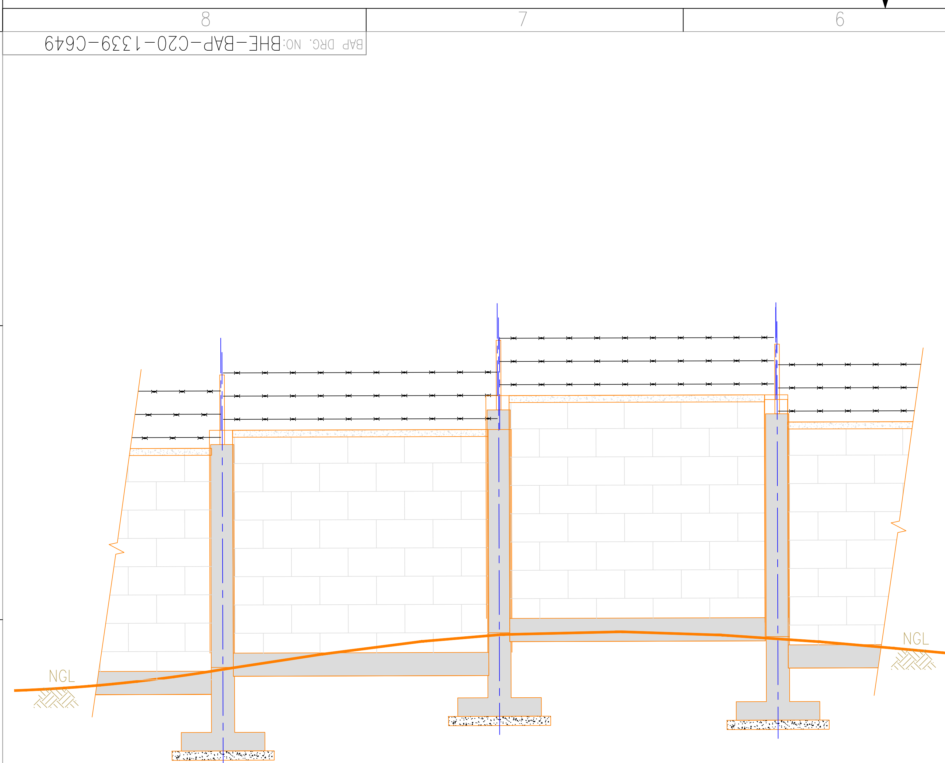
TYPICAL SECTION AT UNDULATED GROUND
