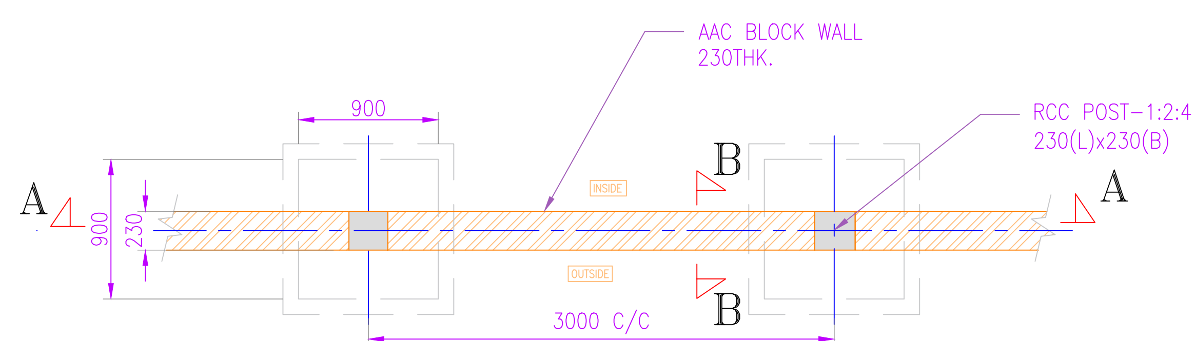
PLAN SCALE 1:50
