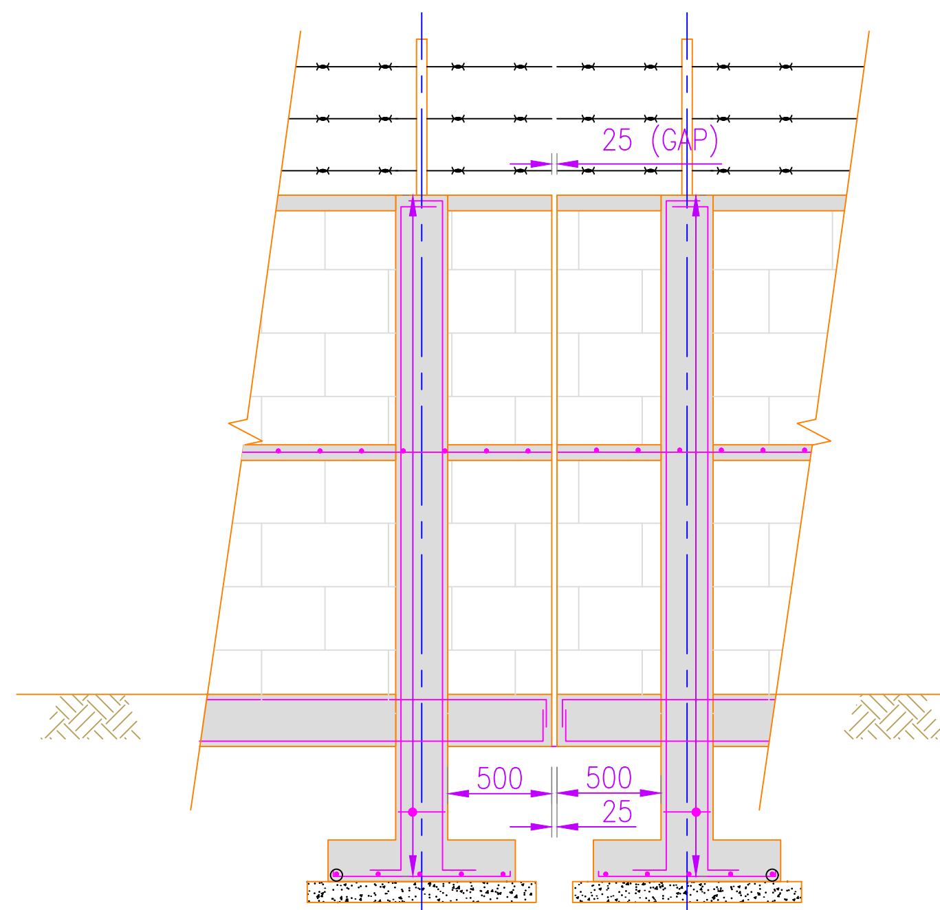
TYPICAL SECTION AT EXPANSION JOINT (at every 30m length)
