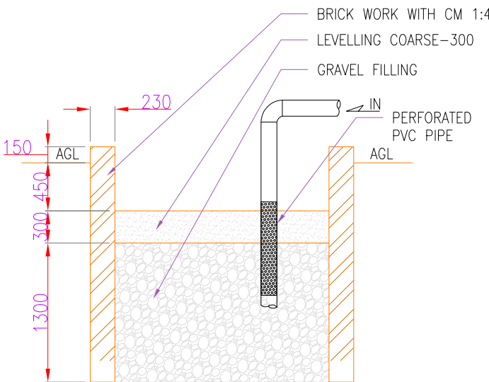
SECTION (TYP) SCALE 1:50
