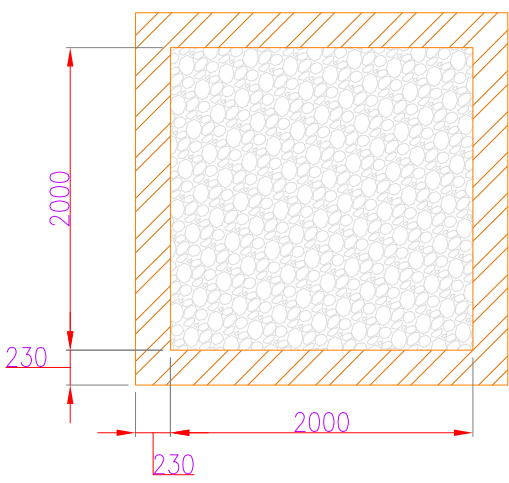
PLAN (TYP) SCALE 1:50
