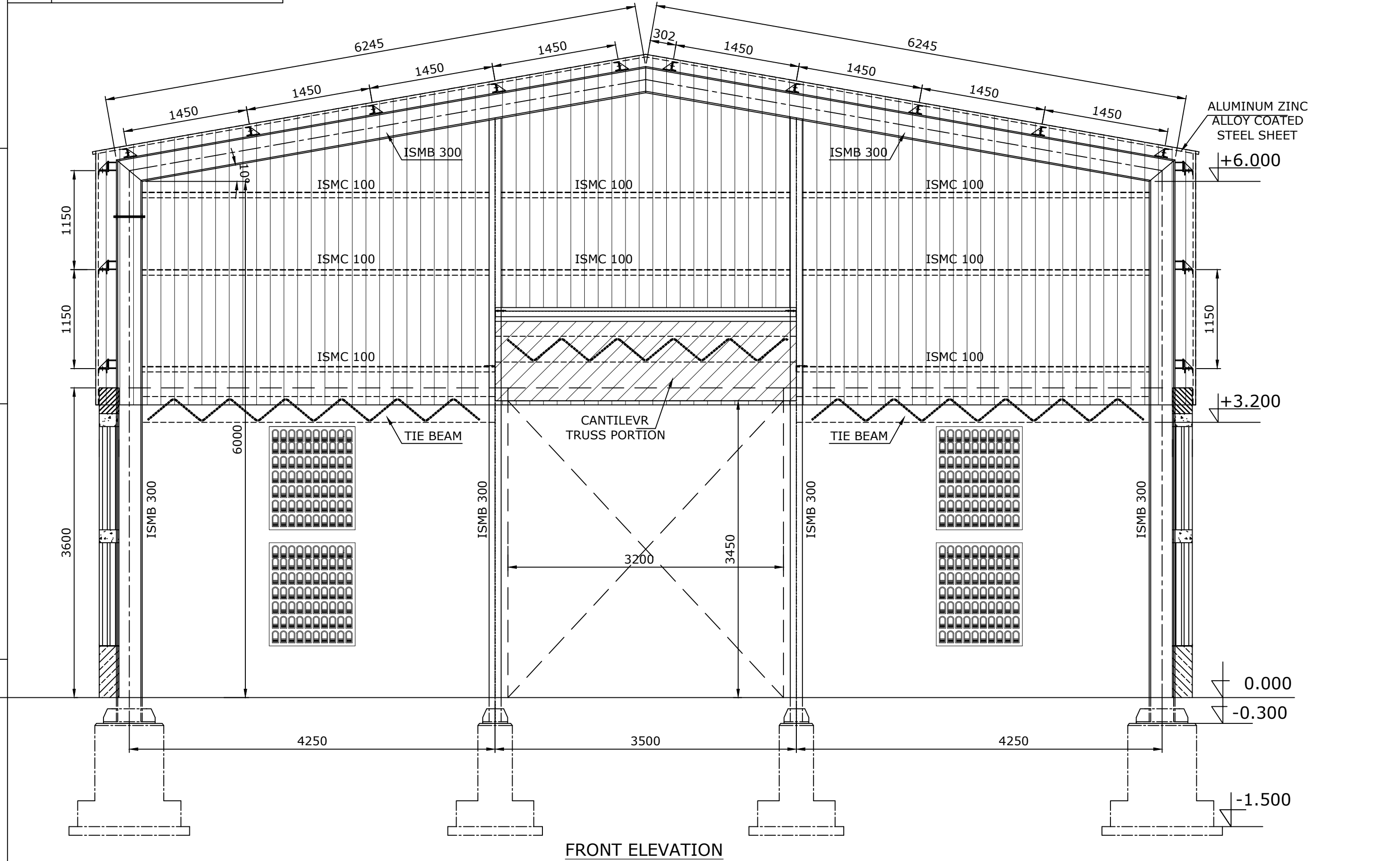
FRONT ELEVATION
