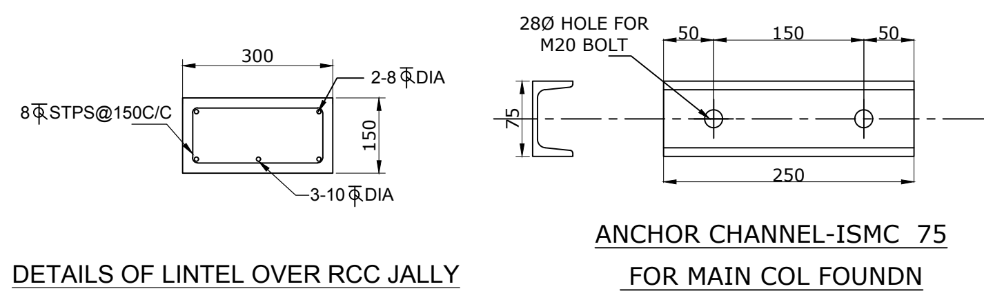
DETAILS OF LINTEL OVER RCC JALLY
