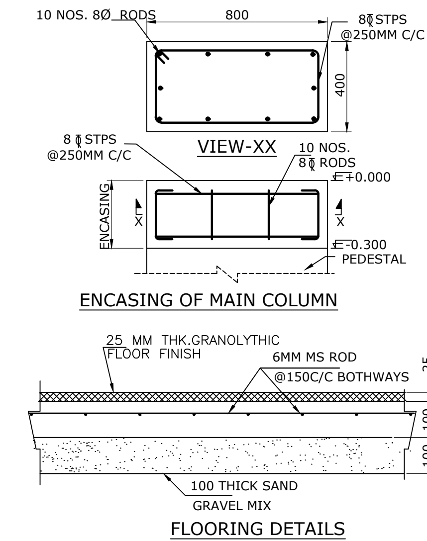
FLOORING DETAILS
