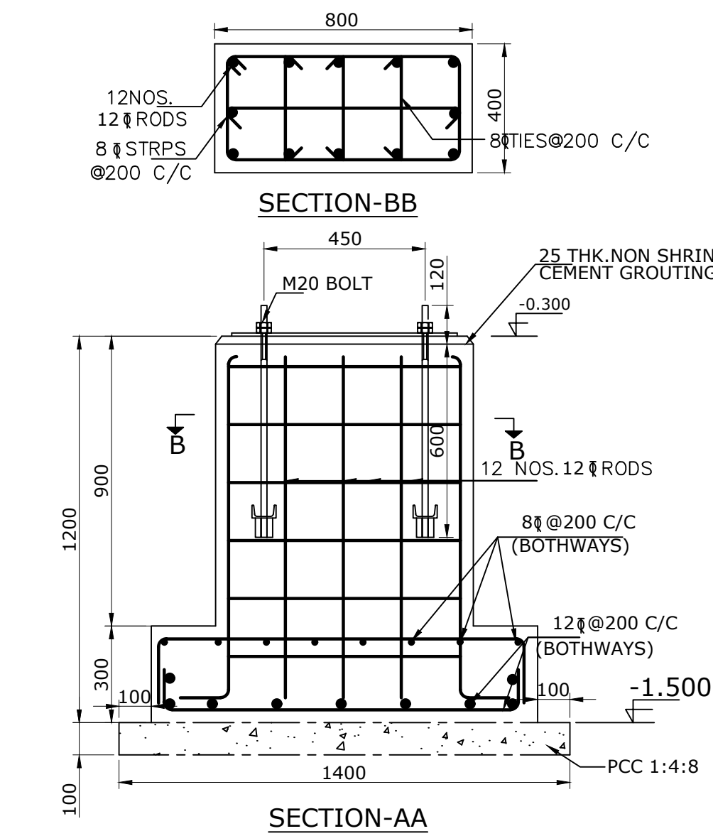
SECTION-AA
