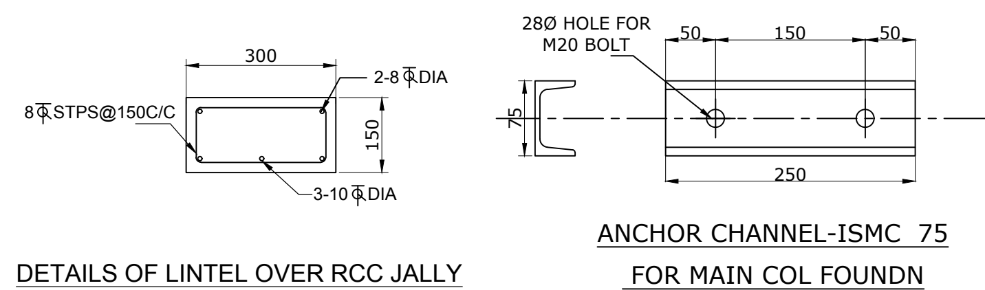
DETAILS OF LINTEL OVER RCC JALLY
