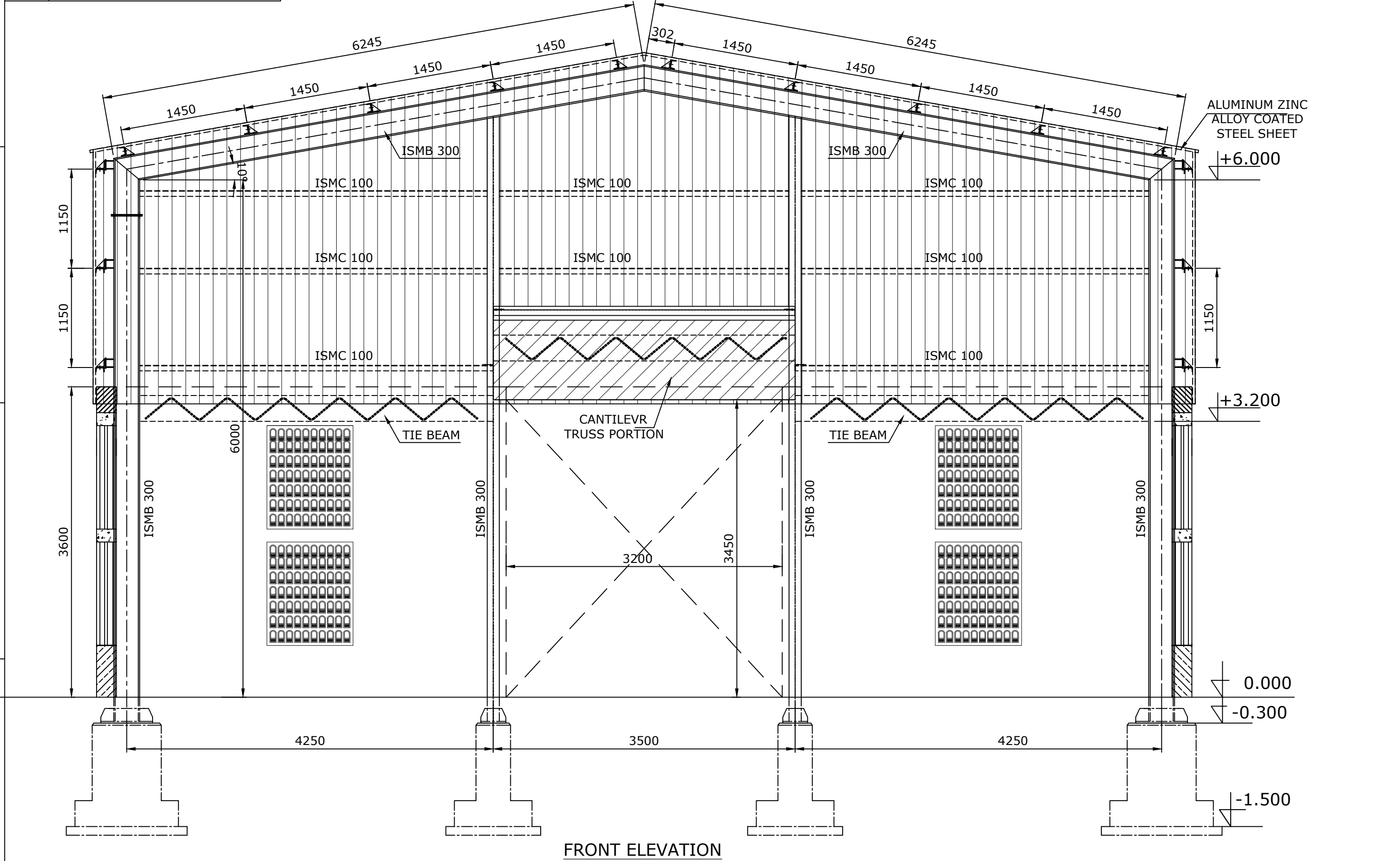
FRONT ELEVATION
