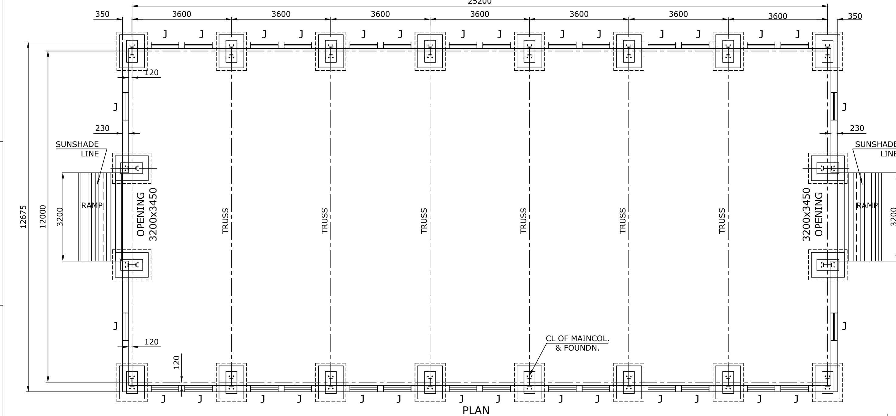
PLAN
