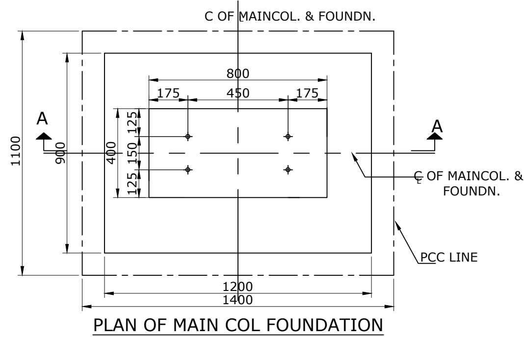
PLAN OF MAIN COL FOUNDATION
