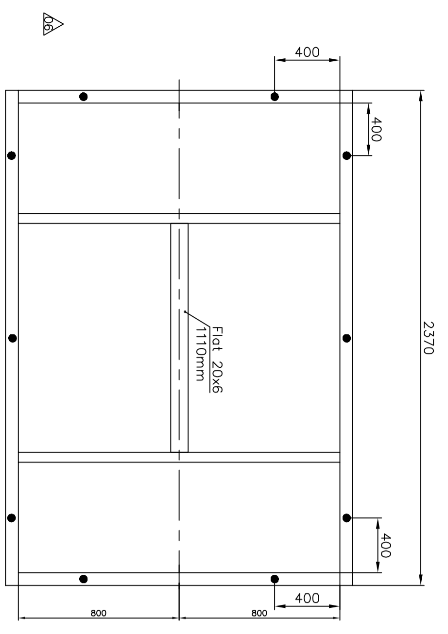
TOP VIEW
