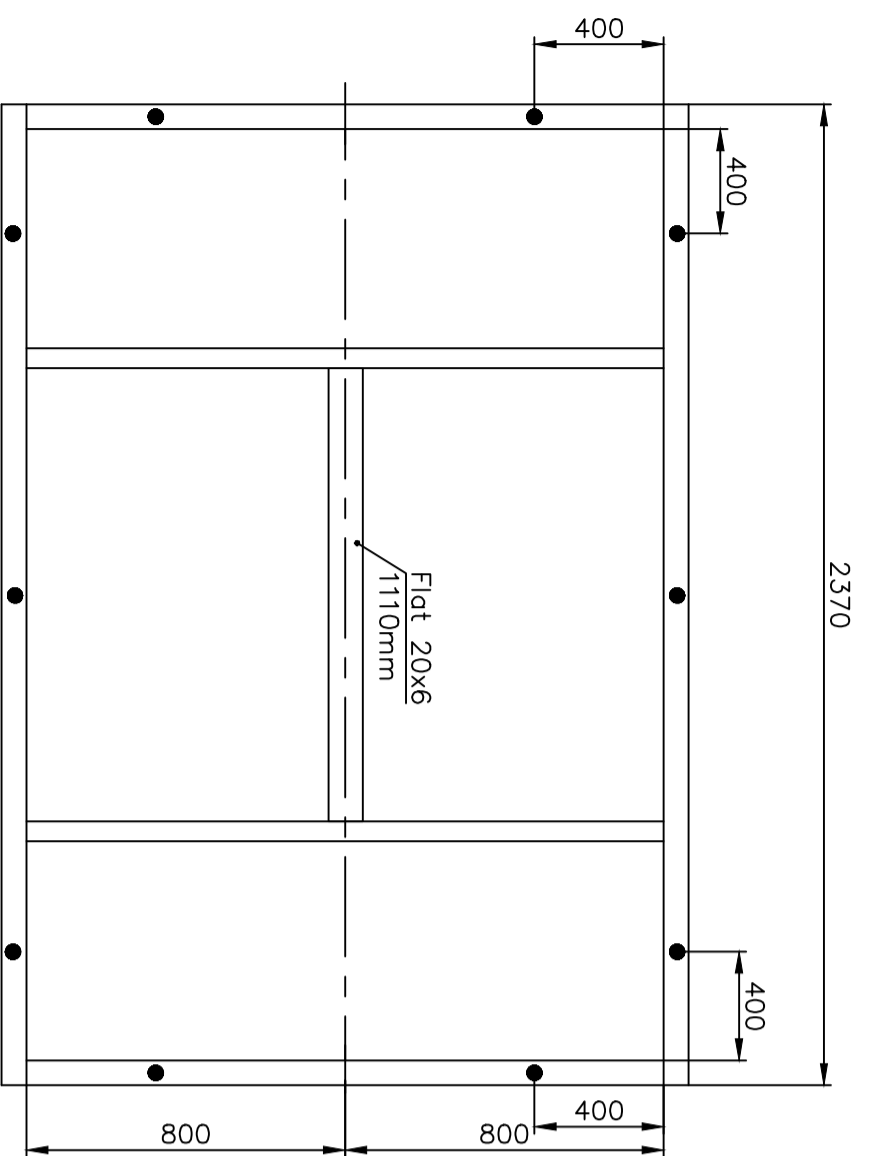
TOP VIEW
