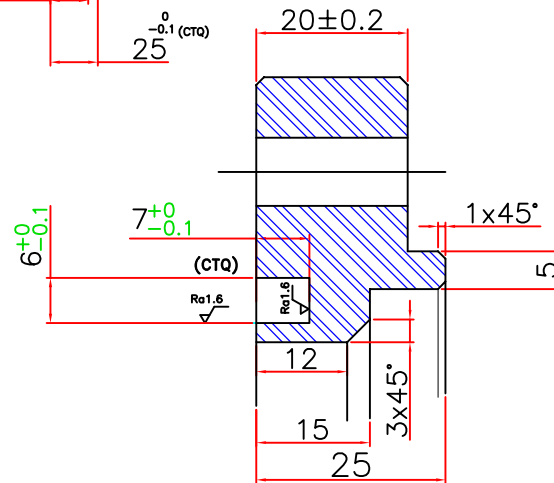
ENLARGED DETAIL-X
