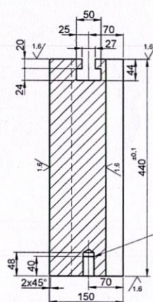
SECTION-BB (SCALE 1:5)
