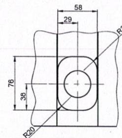
VIEW-X (SCALE 1:2.5)
