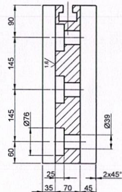
SECTION-AA (SCALE 1:5)
