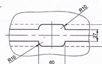
DETAIL-Y (SCALE 1:2.5)
