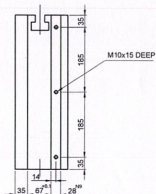
VIEW-Z (SCALE 1:5)
