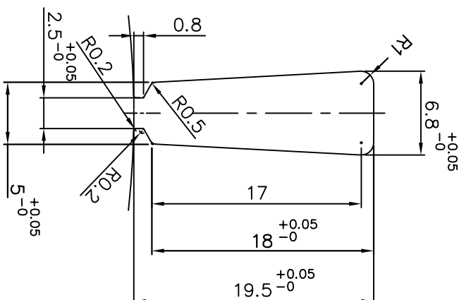
DETAIL-'X'
