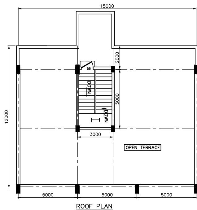
ROOF PLAN
