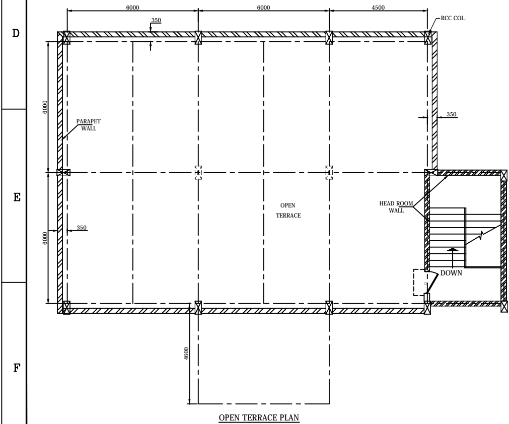
OPEN TERRACE PLAN
