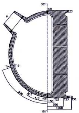
SECTION AT 151'-331'
