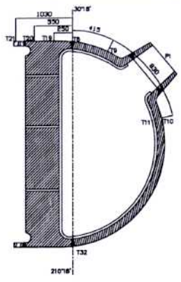
SECTION AT 30'18"-210'18"
