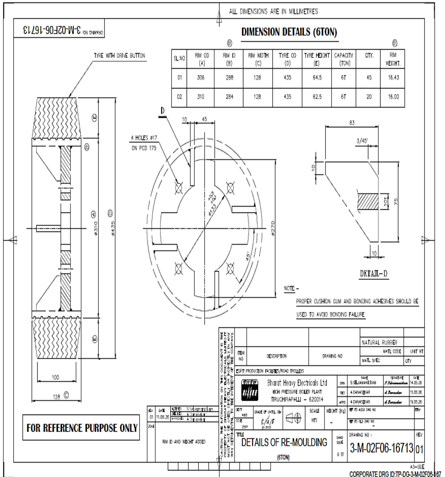
Drawing 3-M-02F06-16713/Rev 01
