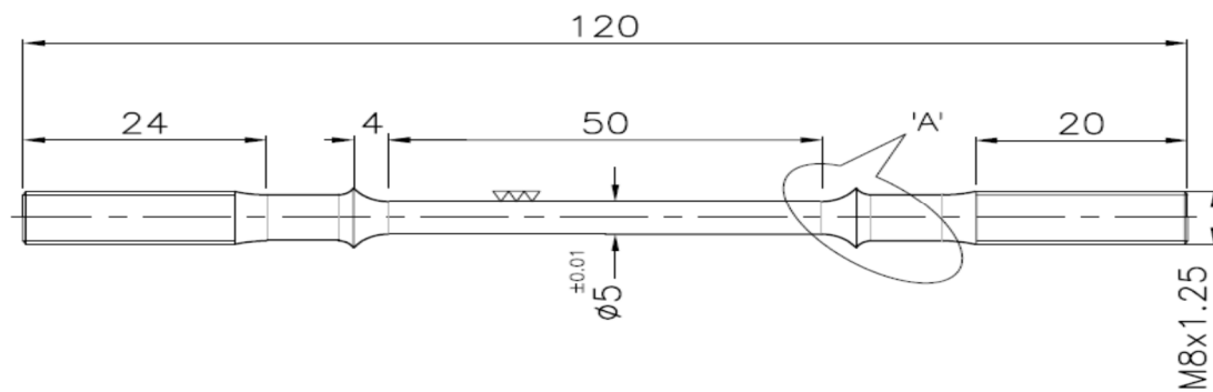
M8 Sample for Creep testing:
