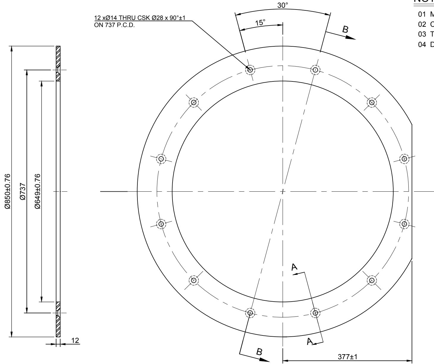
SECTION B-B
