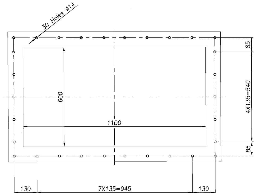
OUTLET FLANGE DETAIL.
