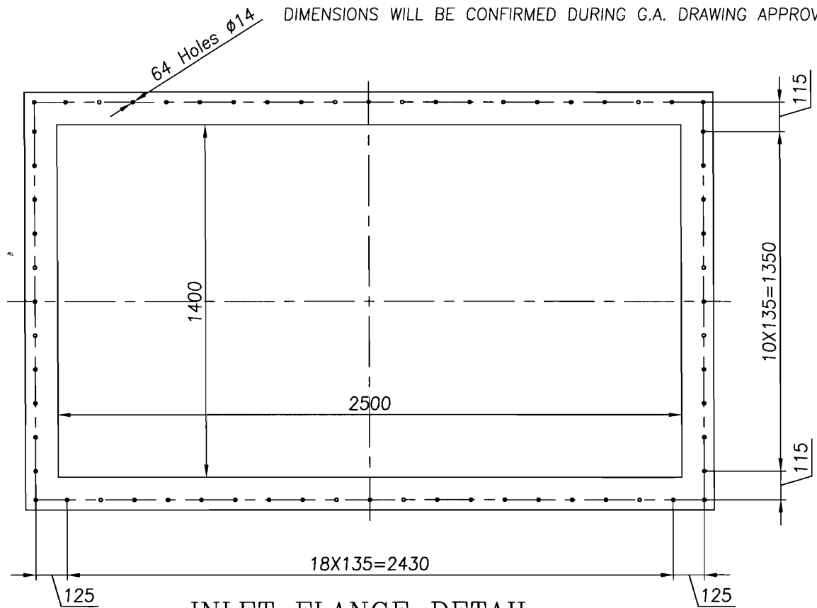
INLET FLANGE DETAIL.
