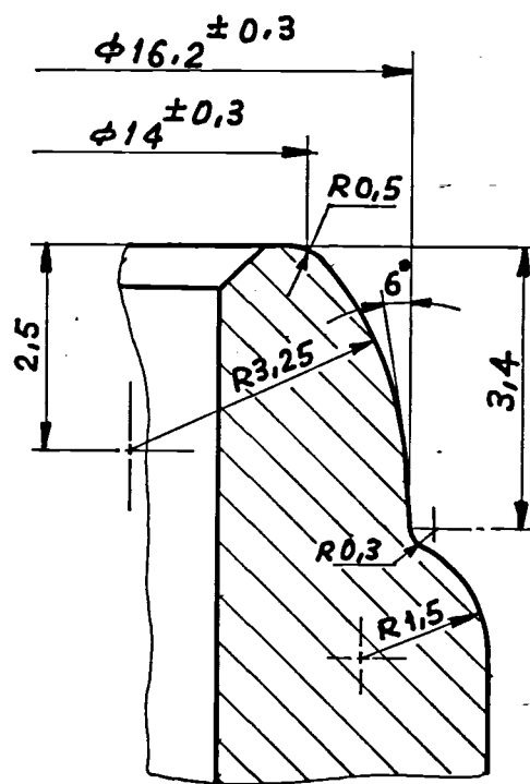
DETAIL - A
