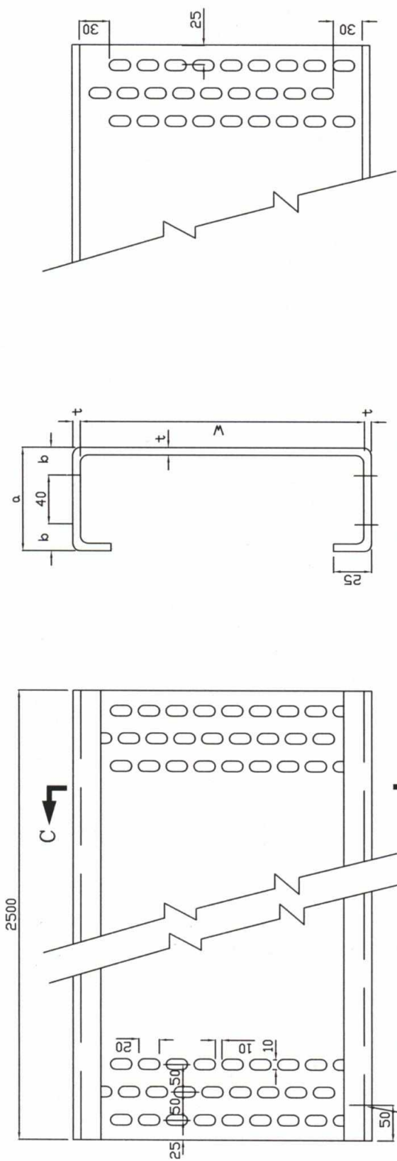
SECTION - CC
