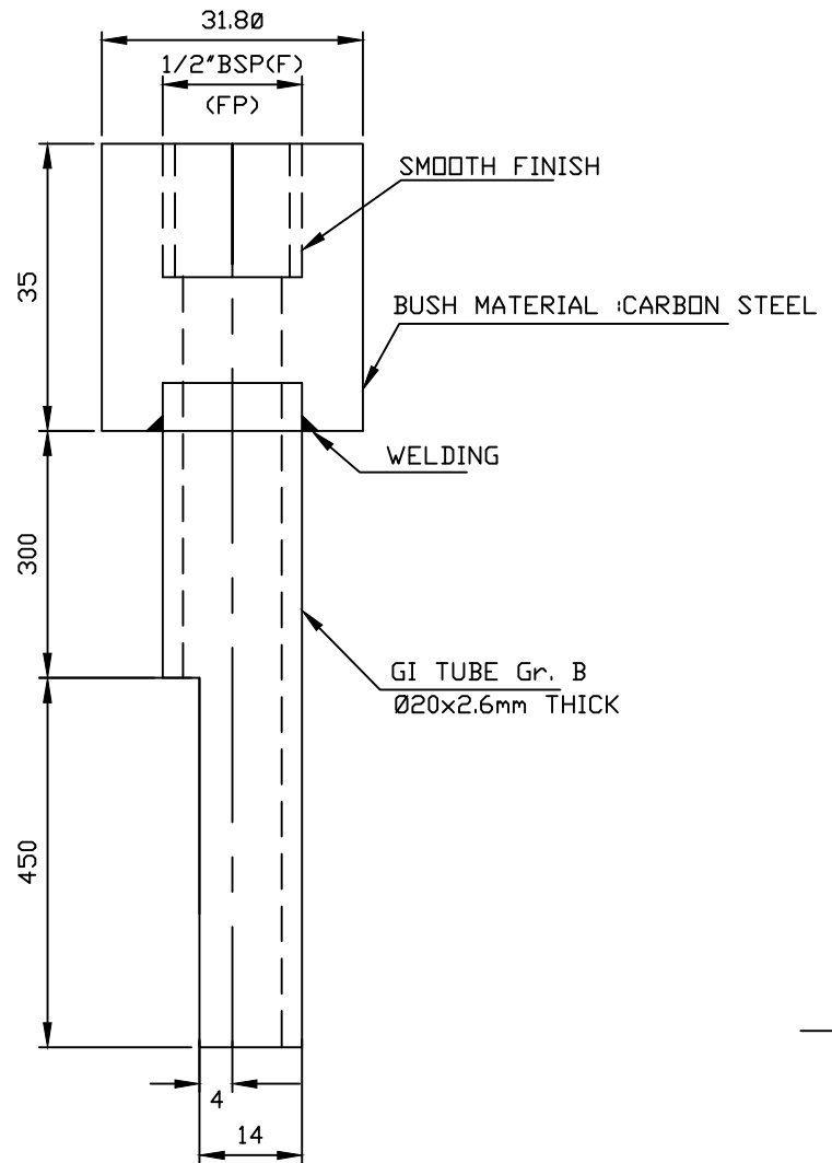
ADAPTOR
