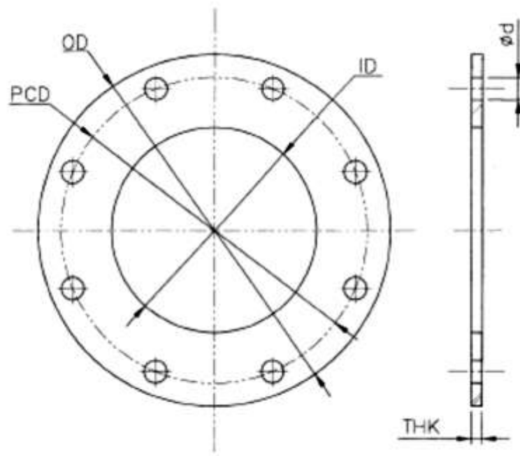
RUBBER GASKET
