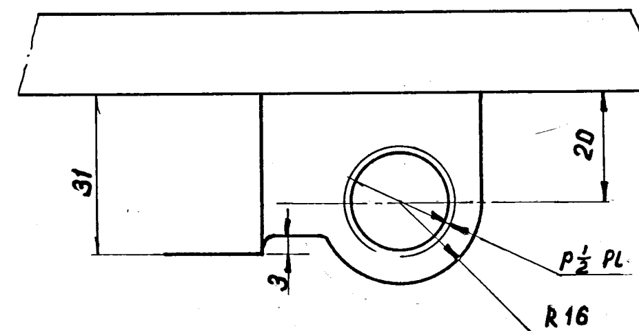
VIEW - A
