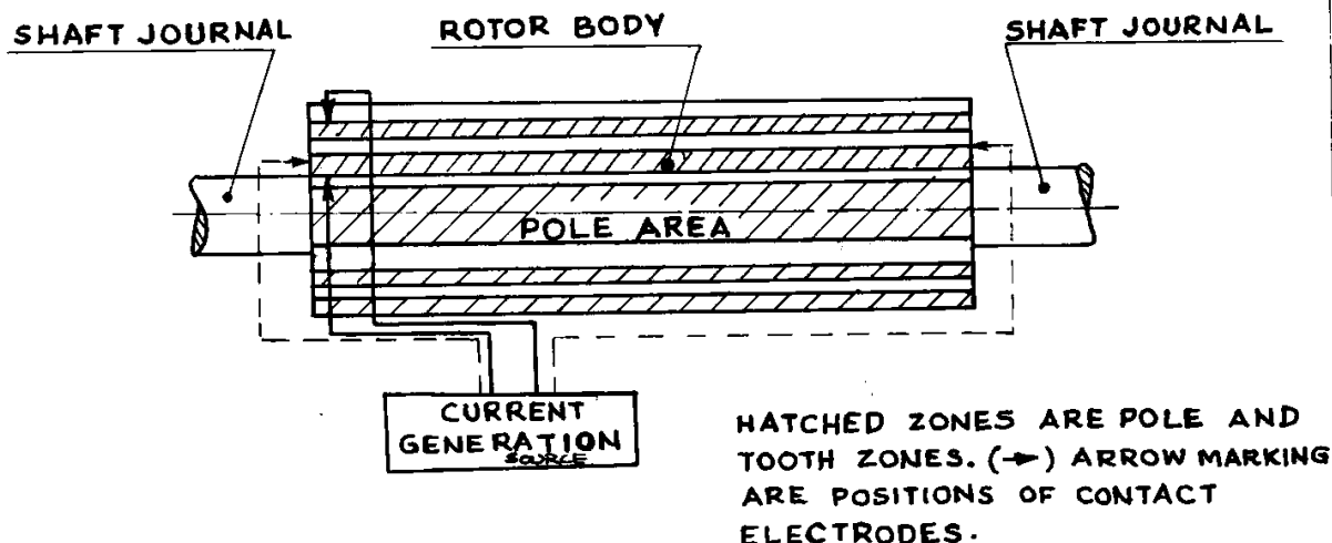
FIG 1: Test setup principle.
