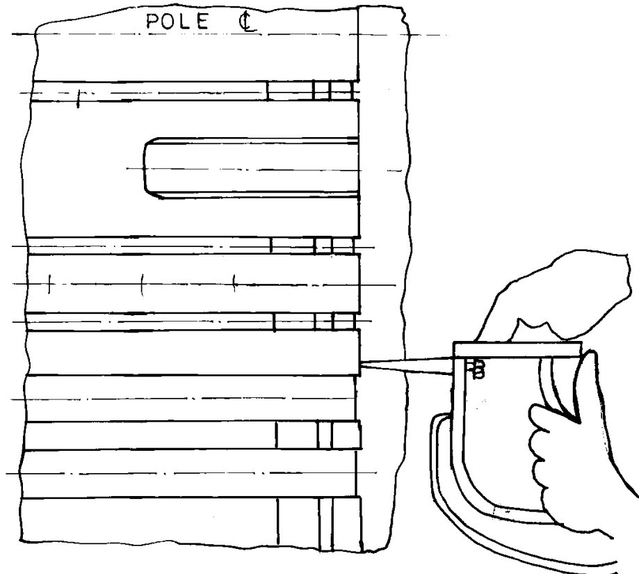
FIG 4: Arrangement of placement of contact electrodes for the testing of axially oriented surface flaws.
