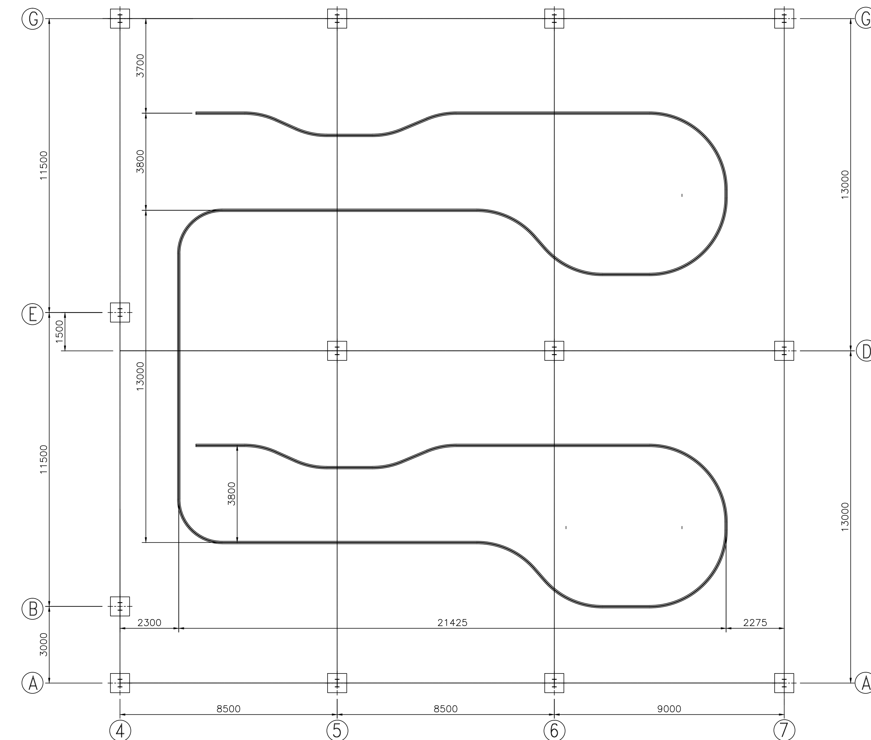
PLAN VIEW OF EL(+) 15.45M (T.O.RCC) MONORAIL PROFILE
