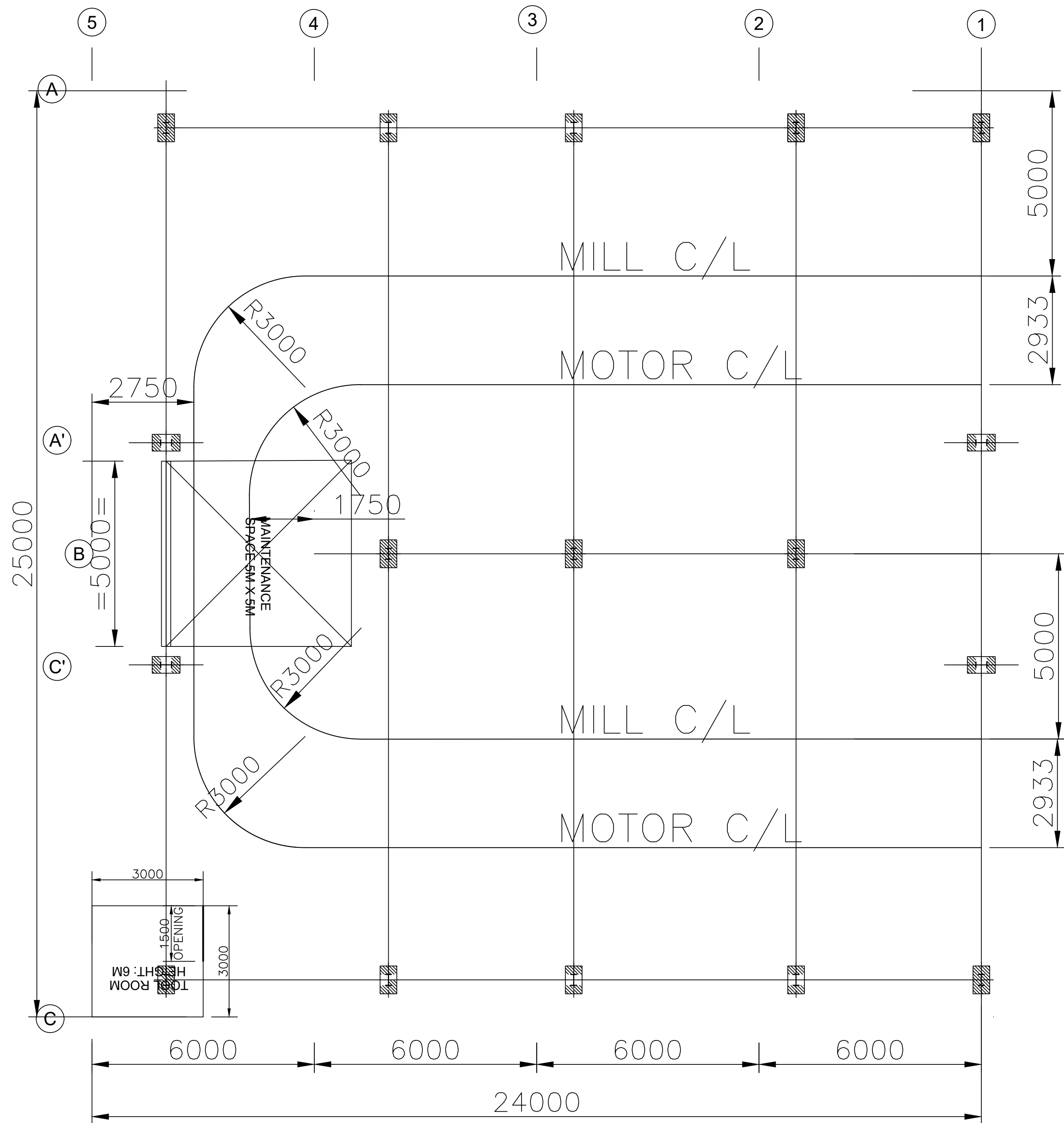
MONORAIL PROFILE
