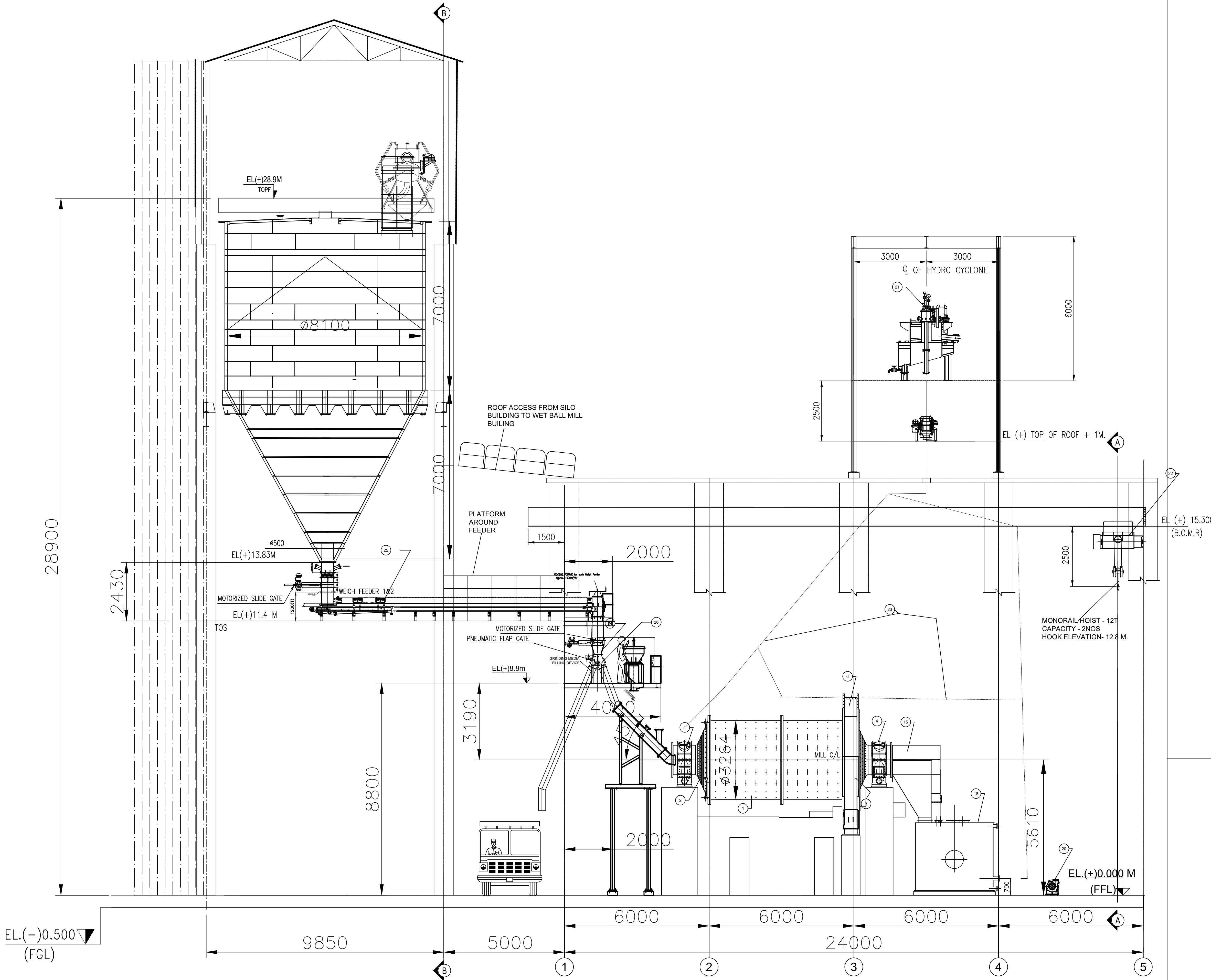
VIEW A
