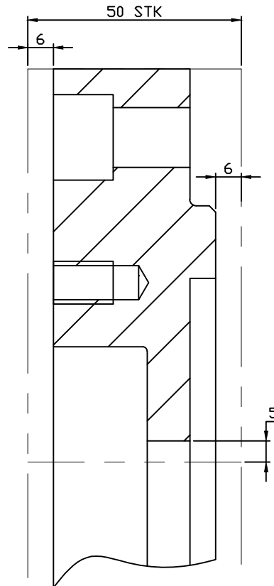
MACHINING ALLOWANCES
