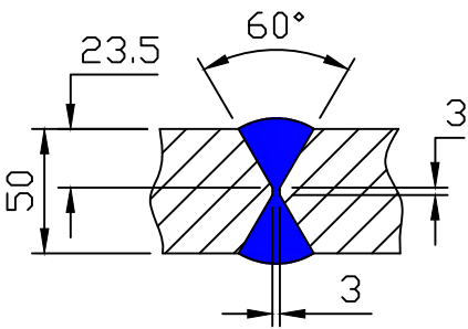
W.P.S NO. WE 001 SECTION: B-B EDGE PREPARATION SCALE 1:3
