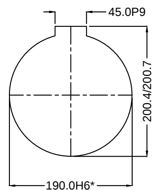
Detail of spigot on hub
