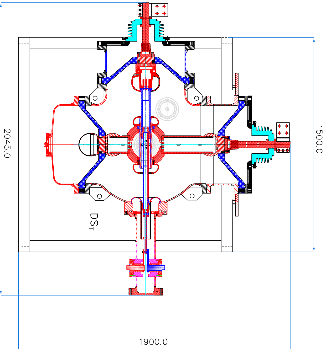
FIGURE 3. BUS TRANSFER CURRENT TEST ON 420 kV GAS DISCONNECTOR SWITCH
