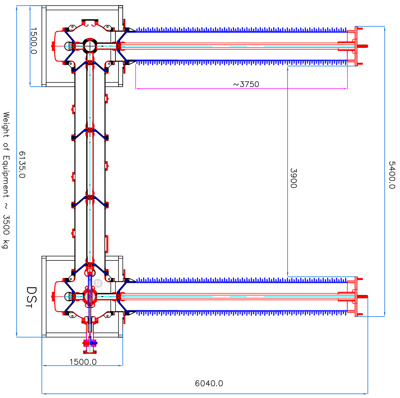
Figure 2. CURRENT SWITCHING CAPABILITY TEST BUS CHARGING CURRENT TEST
