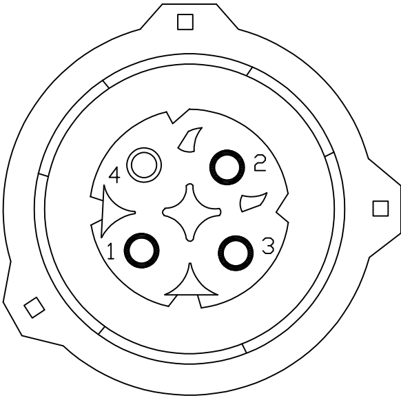
VIEW - X
