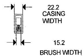
VIEW A BRUSH END VIEW (TYP.)
