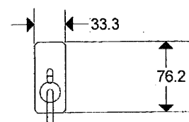
VIEW B WINDOW END VIEW (TYP.)
